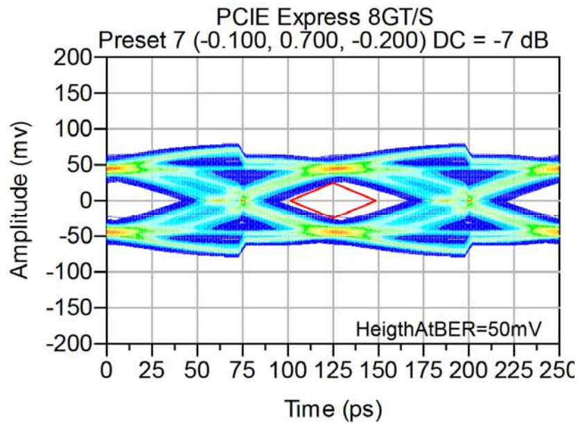
Figure 9 - 8.0 GT/s Eye (21" Tx board trace, 4" Rx board trace)
