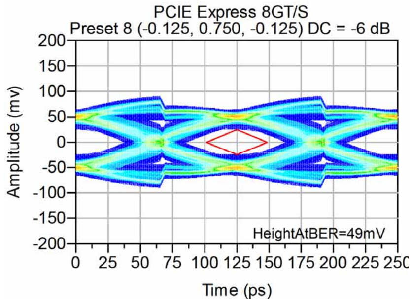
Figure 10 - 8.0 GT/s Eye (21" Tx board trace, 4" Rx board trace, with 200 nF DC blocking Capacitor)
