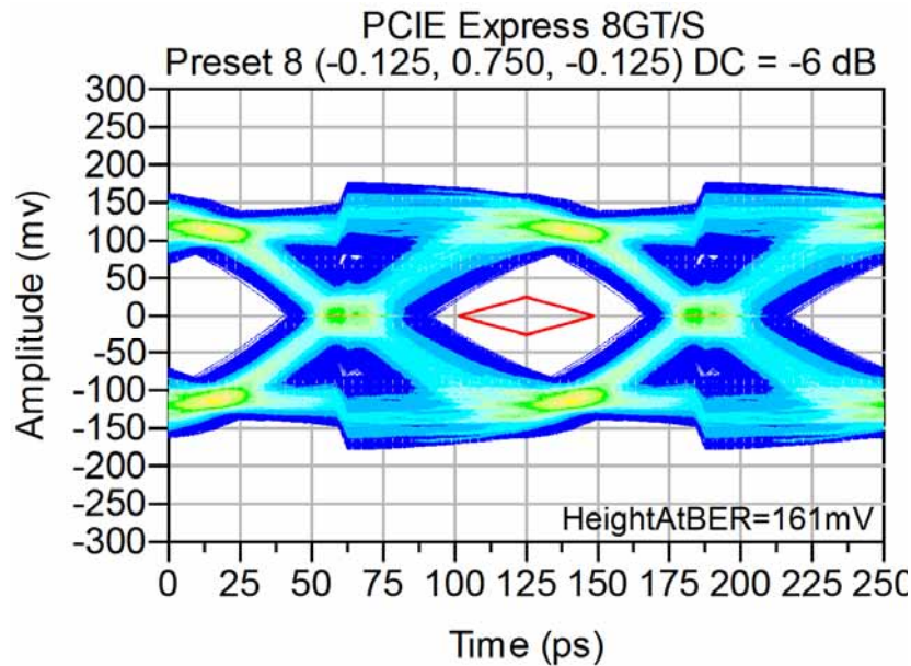
Figure 11 - 8.0 GT/s Eye (0.2" Tx board trace, 0.2" Rx board trace)
