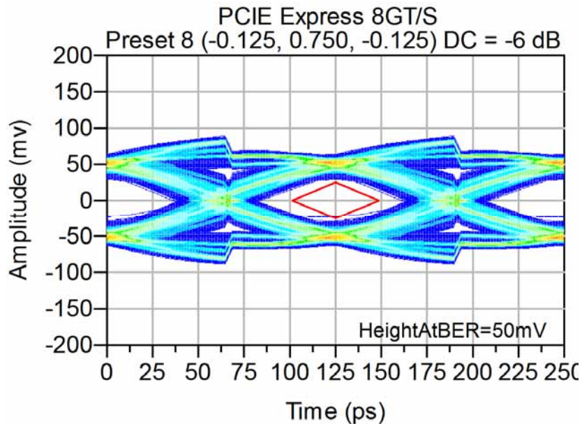
Figure 14 - 85 Ohm System 8.0 GT/s Eye (21.5" Tx board trace, 4" Rx board trace, with 200 nF DC blocking Capacitor)
