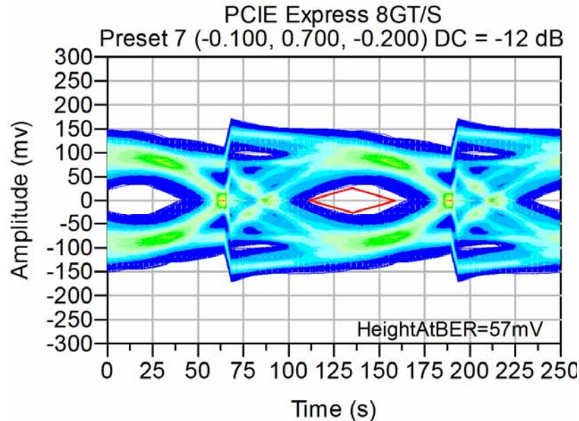
Figure 12 - 8.0 GT/s Eye (0.1" Tx board trace, 0.9" Rx board trace)
