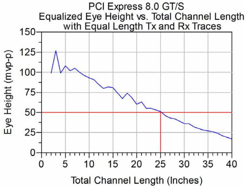
Figure 4 - 8.0 GT/s Eye Height vs. Length
