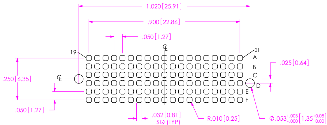
RECOMMENDED STENCIL LAYOUT STENCIL TO BE .0060 [0.152] THICK
