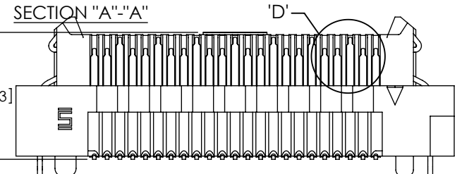
ODD ROW (DP SIDE, HOT PLUG SIDE) (PIN ORIENTATION TO BE EXACTLY AS SHOWN)
