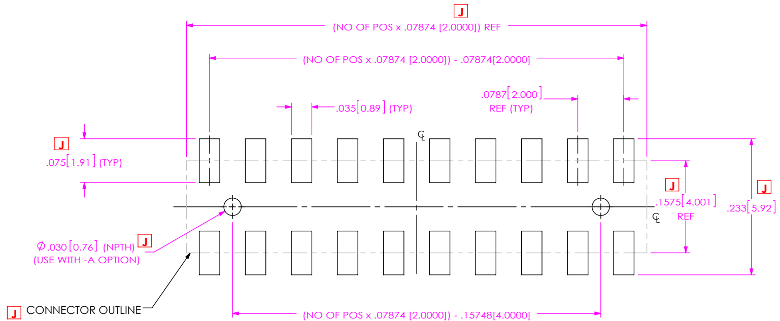
J FIG 1 CLT-110-02-XX-D-A SHOWN ALL DIMENSIONS ARE SYMMETRIC ABOUT THE CENTERLINE
