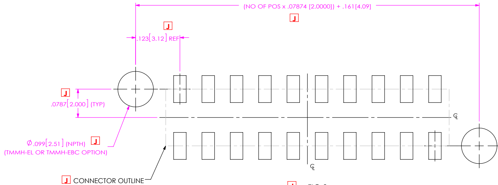
J FIG 2 CLT-110-02-XX-D SHOWN (MATED WITH TMMH-EL OR TMMH-EBC) (SAME AS FIG 1, DIFFERENT AS SHOWN) ALL DIMENSIONS ARE SYMMETRIC ABOUT THE CENTERLINE
