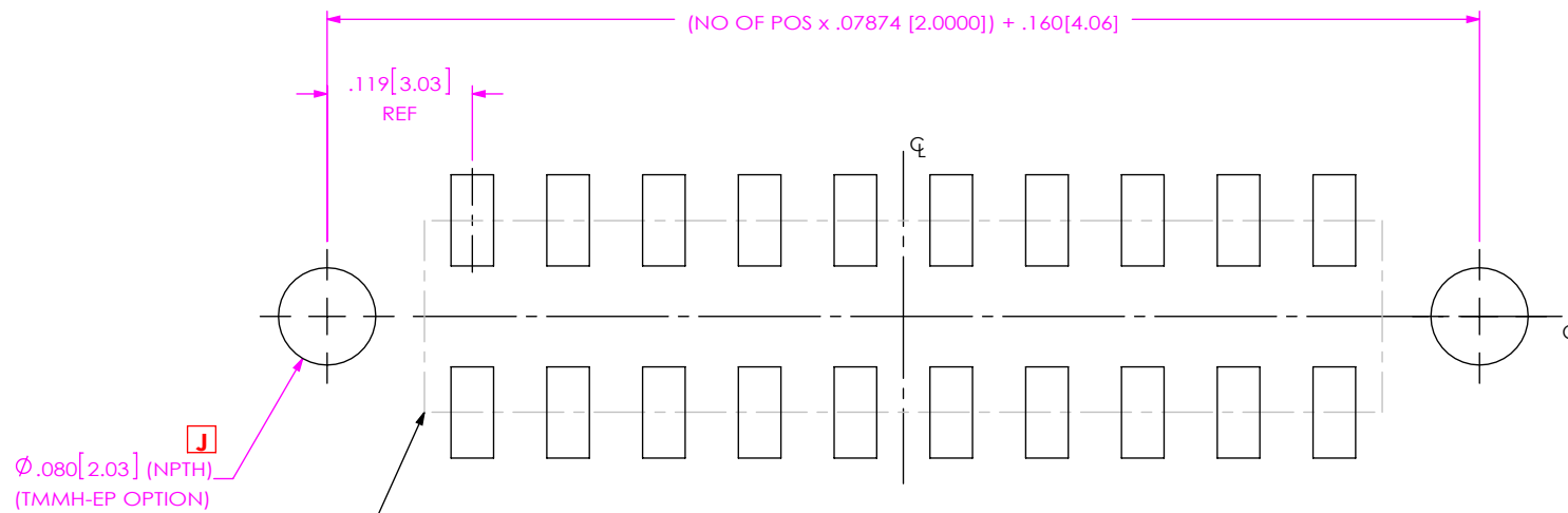
J FIG 3 CLT-110-02-XX-D SHOWN (MATED WITH TMMH-EP) (SAME AS FIG 1, DIFFERENT AS SHOWN) ALL DIMENSIONS ARE SYMMETRIC ABOUT THE CENTERLINE
