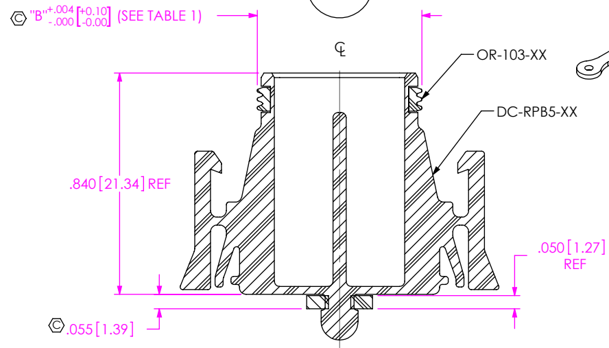
SECTION "B"-"B" SCALE 2 : 1
