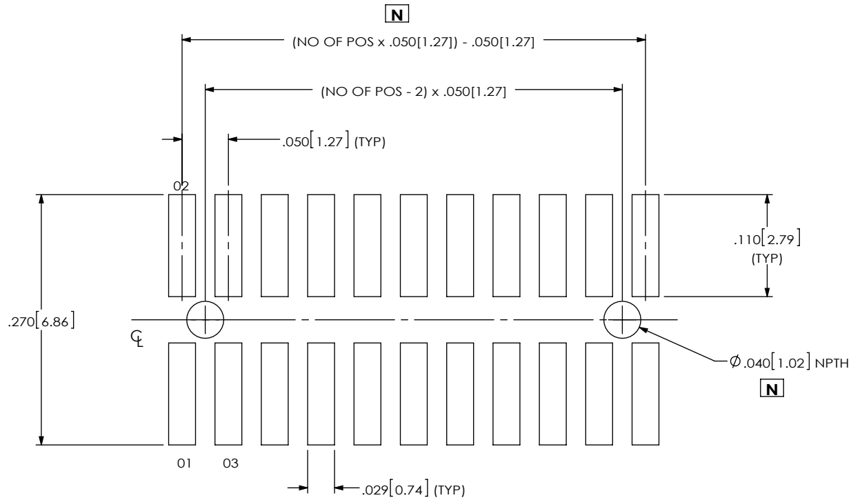
FIG 2 FTS-1XX-XX-XX-DV-A SHOWN ALL DIMENSIONS ARE SYMMETRIC ABOUT THE CENTERLINE
