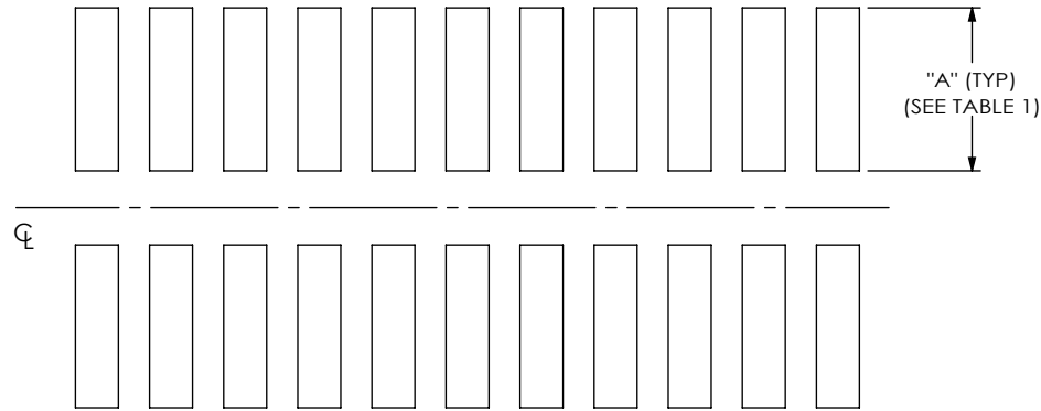
N FIG 4 FTS-1XX-XX-XX-DV-A SHOWN SAME AS FIG 2, DIFFERENT AS SHOWN ALL DIMENSIONS ARE SYMMETRIC ABOUT THE CENTERLINE
