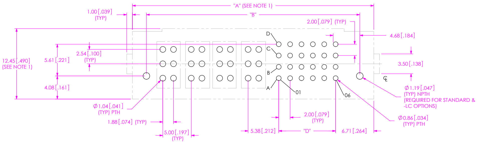
FIG. 2 PCB LAYOUT FOR MPTC-XX-XX-00-6.30-XX-X-V-LC SHOWN
