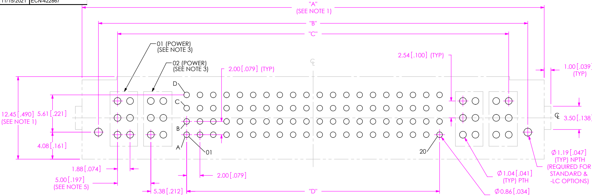
FIG. 1 PCB LAYOUT FOR MPTC-XX-XX-XX-6.30-XX-X-V-LC SHOWN
