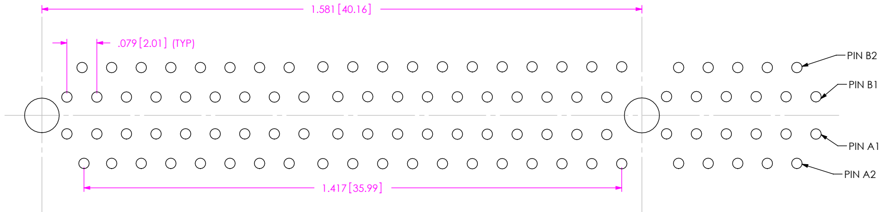
FIG 2 RECOMMENDED PCB LAYOUT (FOR: -098) (SAME AS FIG 1 UNLESS OTHERWISE NOTED)
