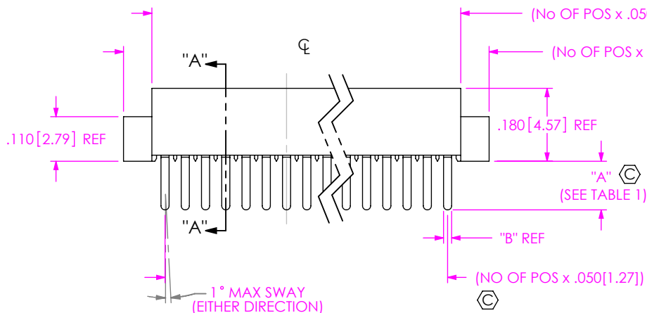
FIG 1 THROUGH HOLE/STRAIGHT MODIFIED
