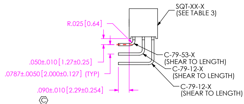
FIG 2 -RA: RIGHT ANGLE (LEAD STYLE -01-S,D,T)
