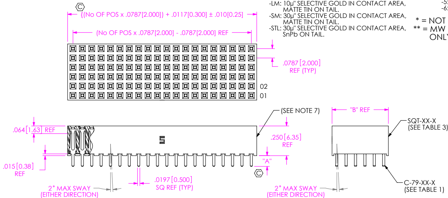
FIG 1 SQT-120-01-XX-6 SHOWN
