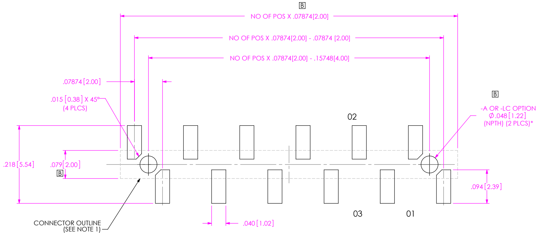
FIG 3 TW-12-XX-X-5-XXX-SM SHOWN * ONLY ONE \varnothing.048 HOLE TO APPEAR ON 02 POSITION
