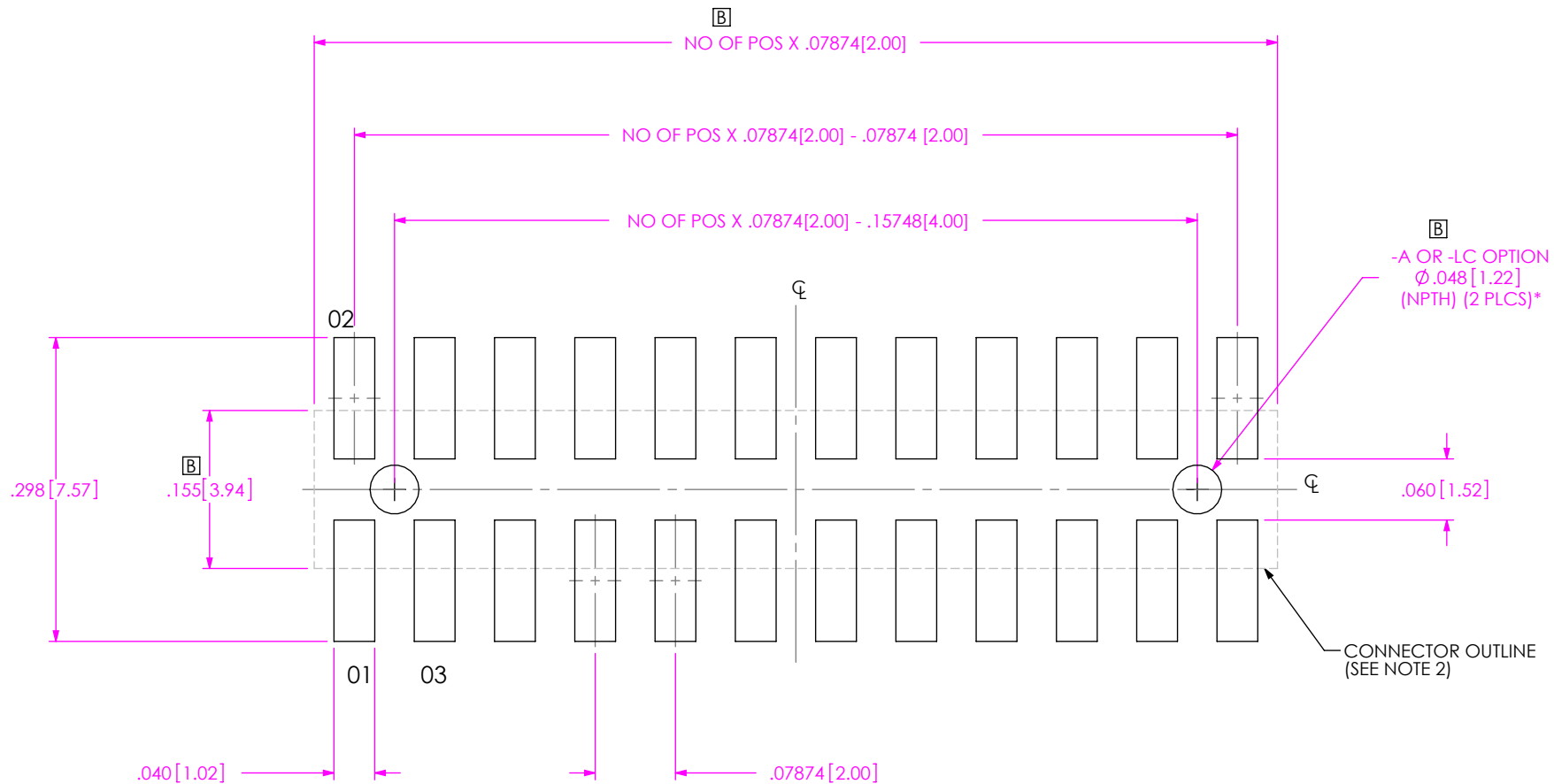
FIG 2 TW-12-XX-X-D-XXX-SM SHOWN * ONLY ONE \text{Ø}.048 HOLE TO APPEAR ON 02 POSITION
