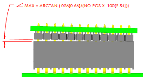
FINAL Y AXIS ANGULAR MISALIGNMENT
