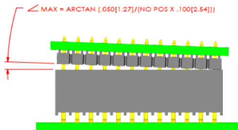
INITIAL Y AXIS ANGULAR MISALIGNMENT
