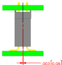
FINAL Y AXIS LINEAR MISALIGNMENT
