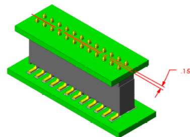
FINAL Z AXIS ANGULAR MISALIGNMENT
