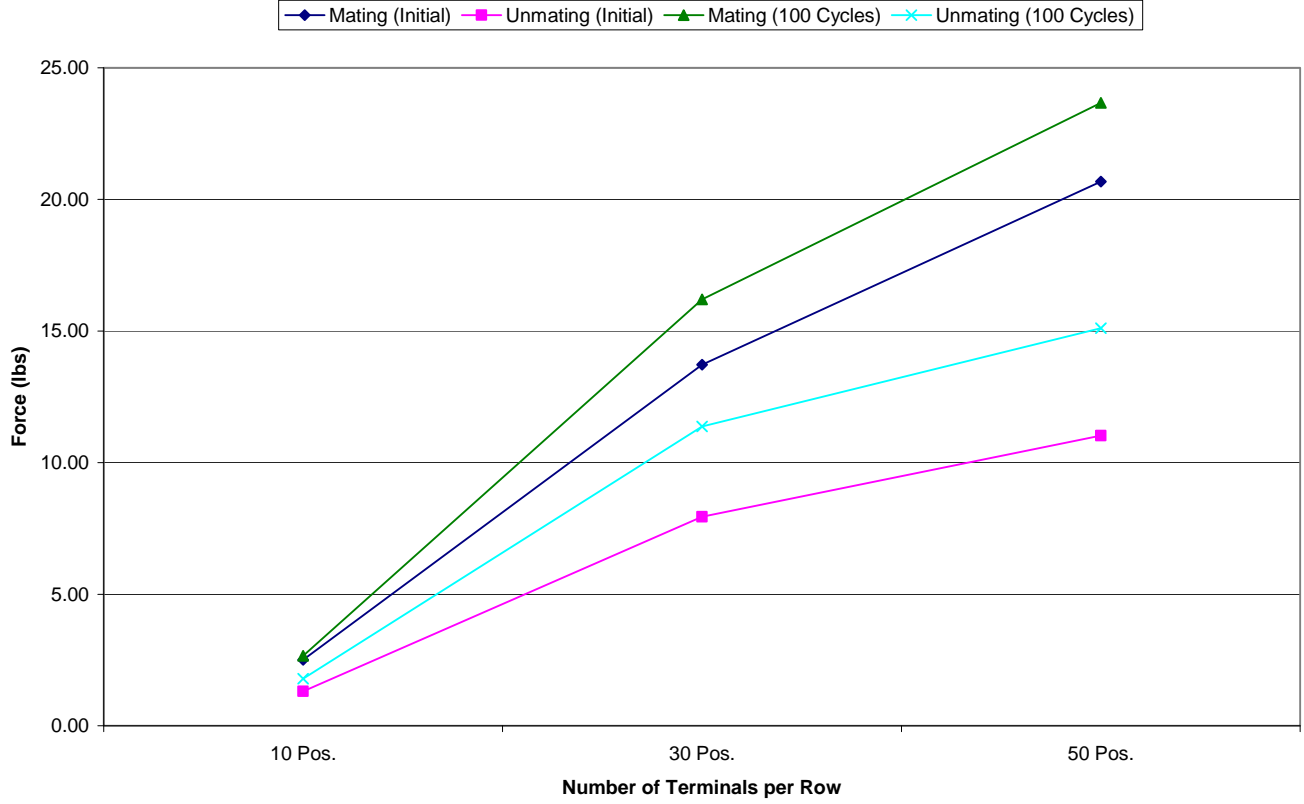
Mating/Unmating Data for 10, 30 and 50 Position SEAF/SEAM
