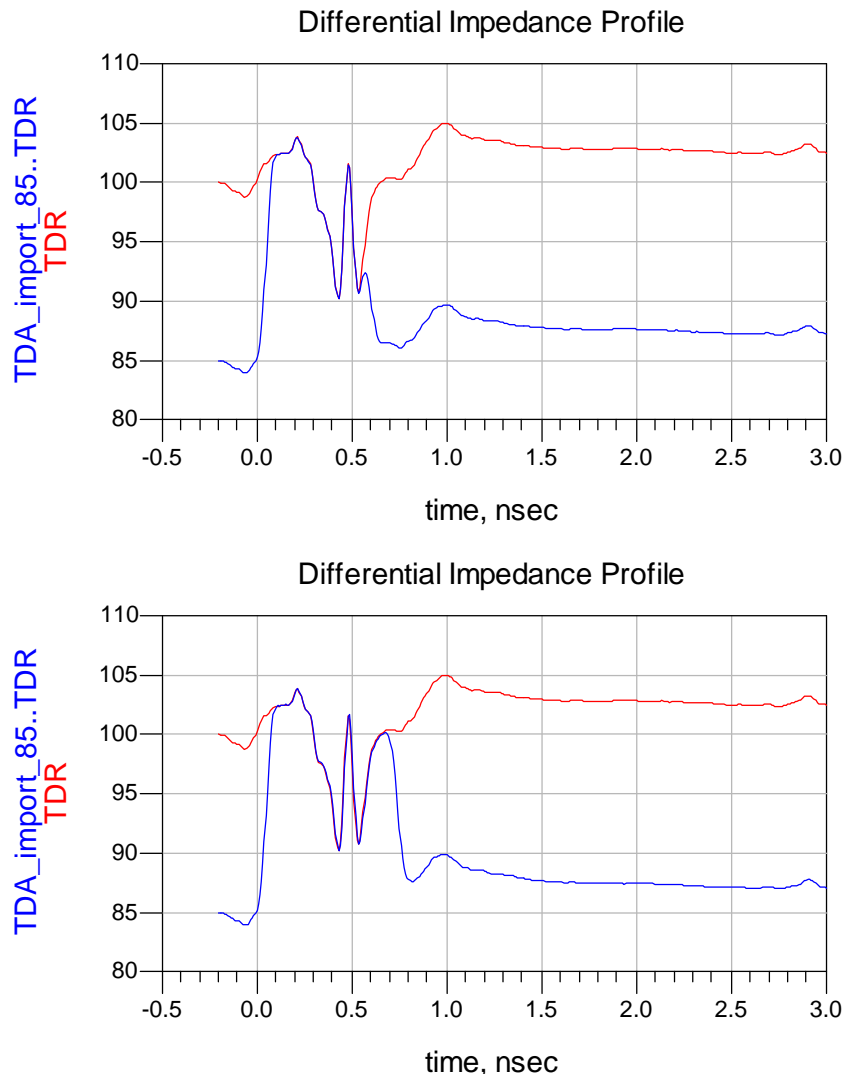
Figure 3. Differential Impedance Profile of 7mm SEAM/SEAF Red – 100 ohm Reference Impedance, Blue – 85 ohm reference Impedance (Optimal Horizontal Routing – Top, Optimal Vertical Routing - Bottom)
