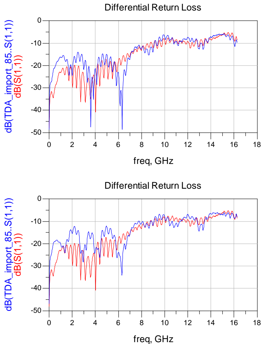
Figure 1. Differential Return Loss of Samtec 7mm SEAM/SEAF Red – 100 ohm Reference Impedance, Blue – 85 ohm reference Impedance (Optimal Horizontal Routing – Top, Optimal Vertical Routing - Bottom)
