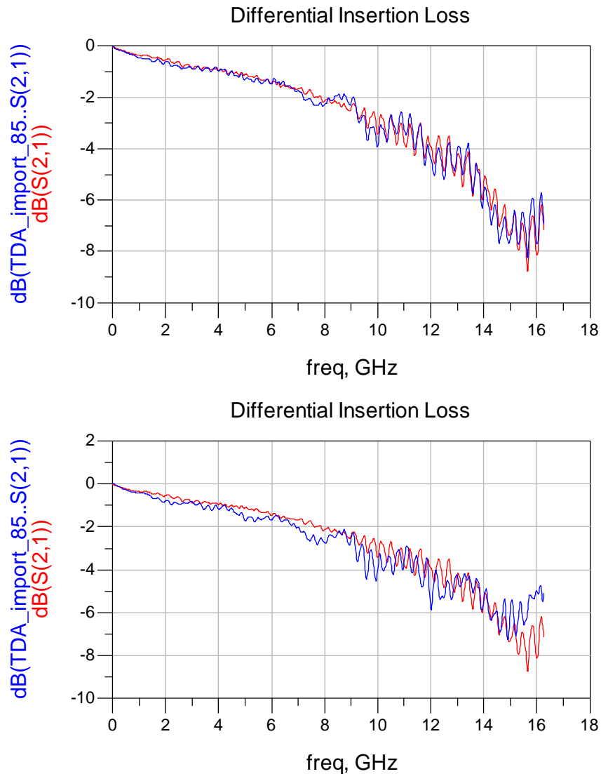
Figure 2. Differential Insertion Loss of Samtec 7mm SEAM/SEAF Red – 100 ohm Reference Impedance, Blue – 85 ohm reference Impedance (Optimal Horizontal Routing – Top, Optimal Vertical Routing - Bottom)
