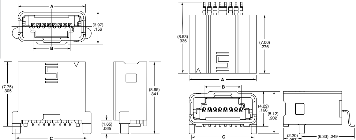
AMF6-02-S-K-XR SHOWN
