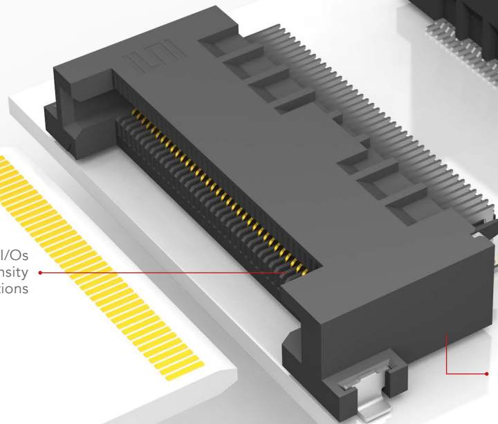
0.80 mm pitch, 140 total positions (MEC8 Series)
