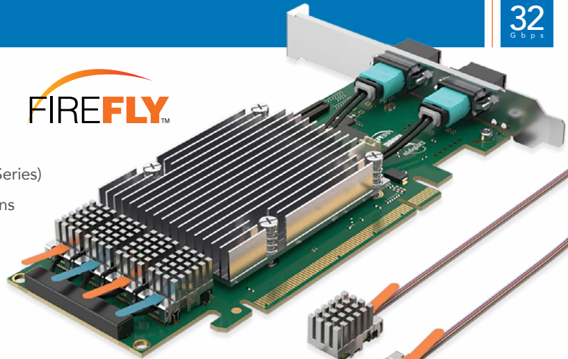
Optical FireFly™ Cables & Adaptor Card
