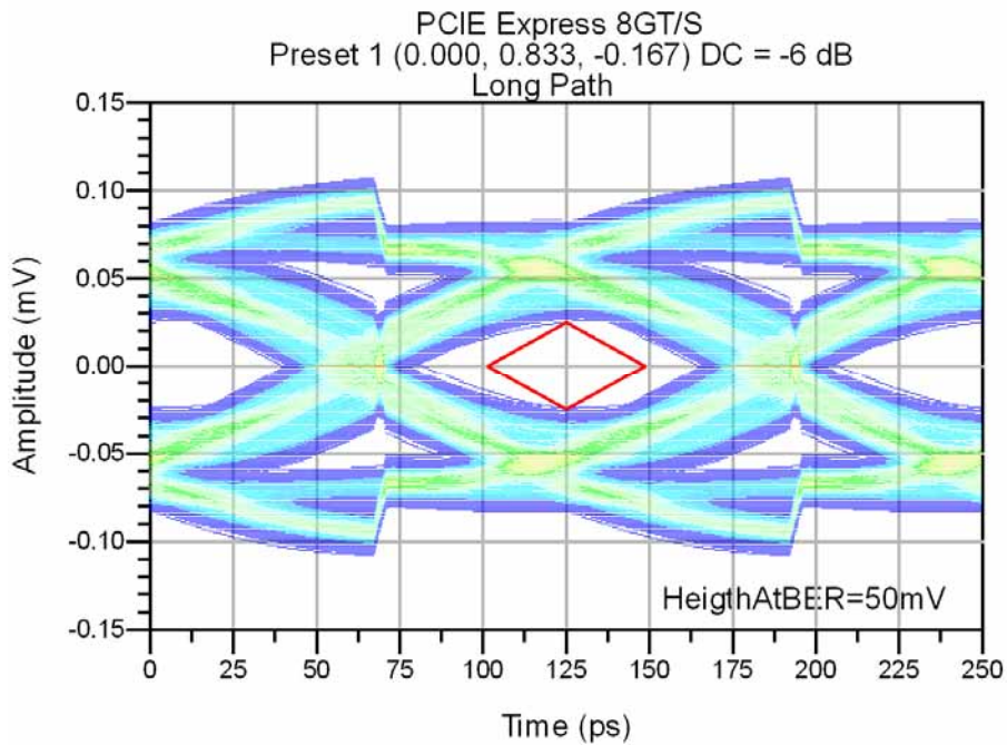
Figure 12 - 8.0 GT/s Eye, Long path (24.0" Tx board trace, 4" Rx board trace)
