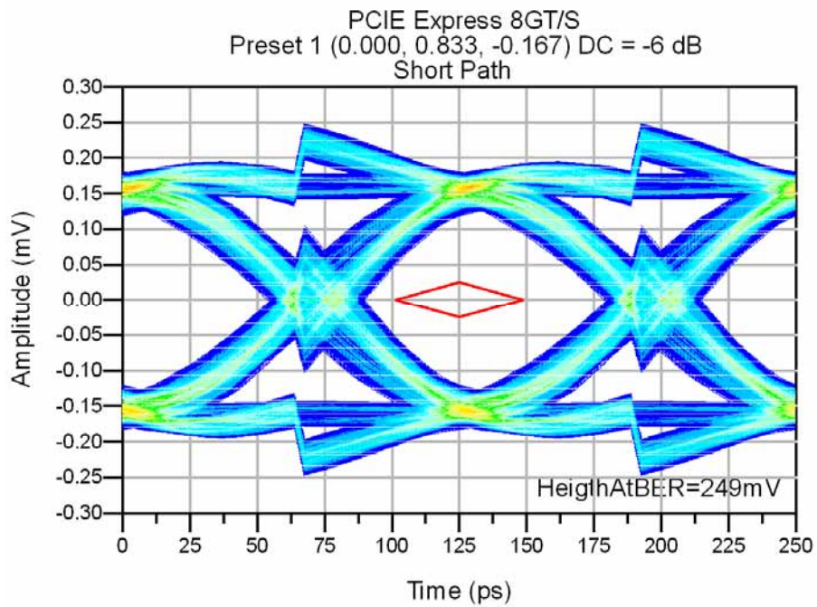
Figure 17 - 8.0 GT/s Eye, Best Case Short Path (0.1" Tx board trace, 0.1" Rx board trace)
