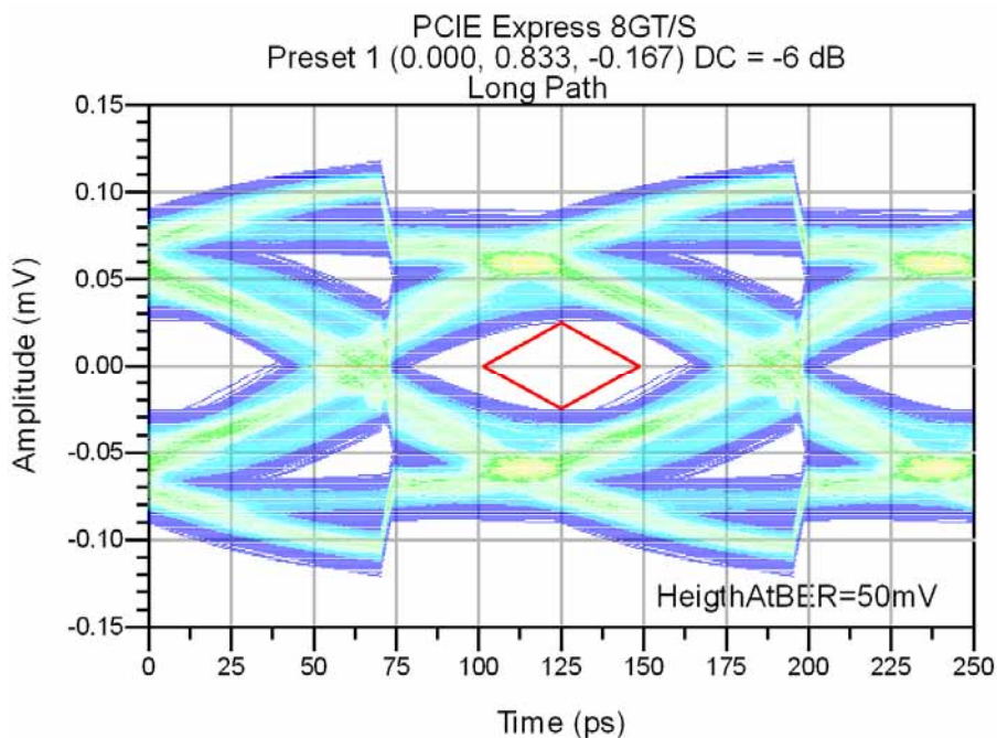
Figure 14 - 8.0 GT/s Eye, Long Path (24.0" Tx board trace, 4" Rx board trace, with 200 nF DC blocking Capacitor)
