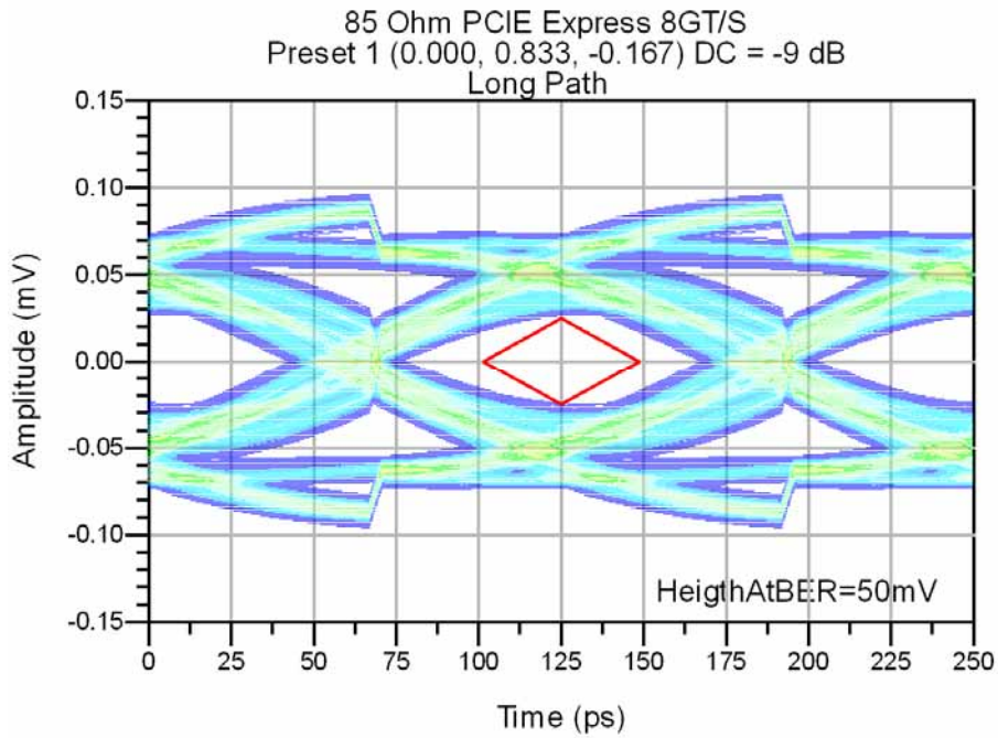
Figure 21 - 85 Ohm System 8.0 GT/s Eye (27.5" Tx board trace, 4" Rx board trace, with 200 nF DC blocking Capacitor)
