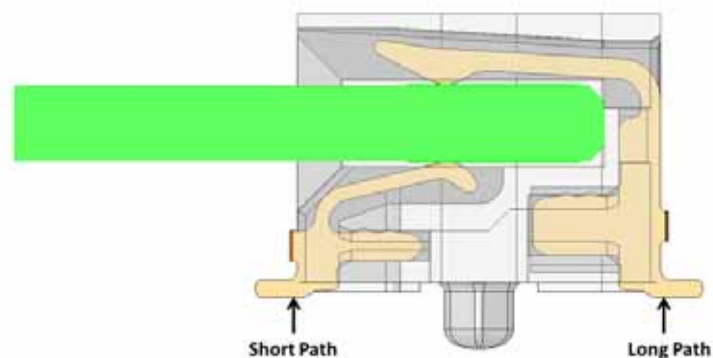
Figure 4 - Side View of MEC6-RA Connector Mated with 0.062" (1.60mm) Edge Card
