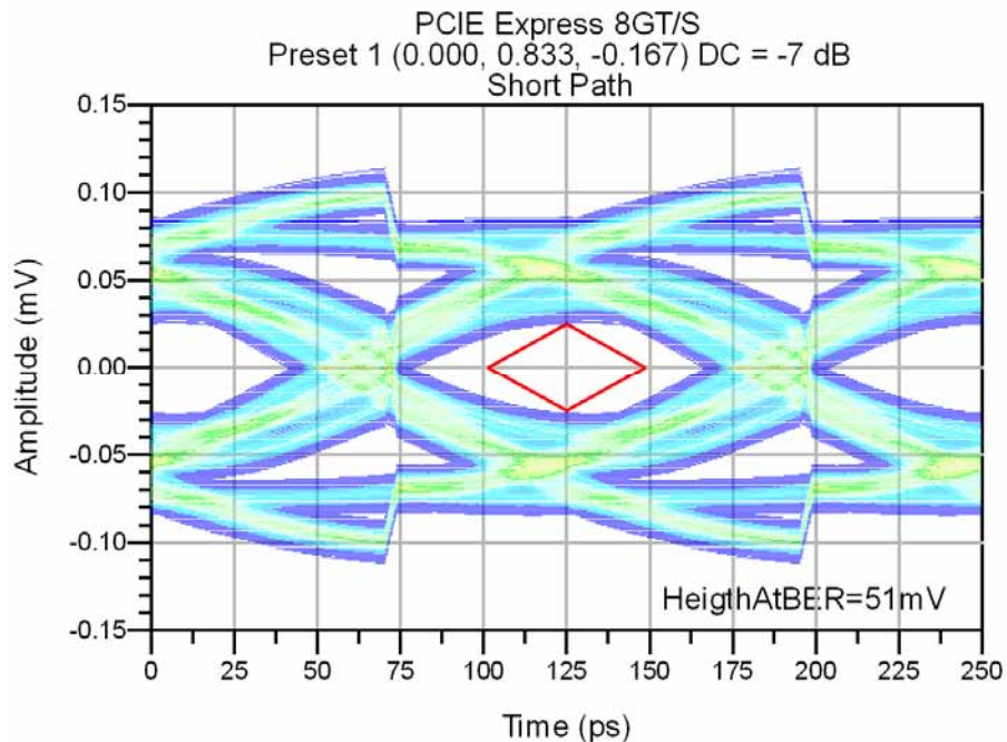
Figure 15 - 8.0 GT/s Eye, Short Path (25" Tx board trace, 4" Rx board trace, with 200 nF DC blocking Capacitor)
