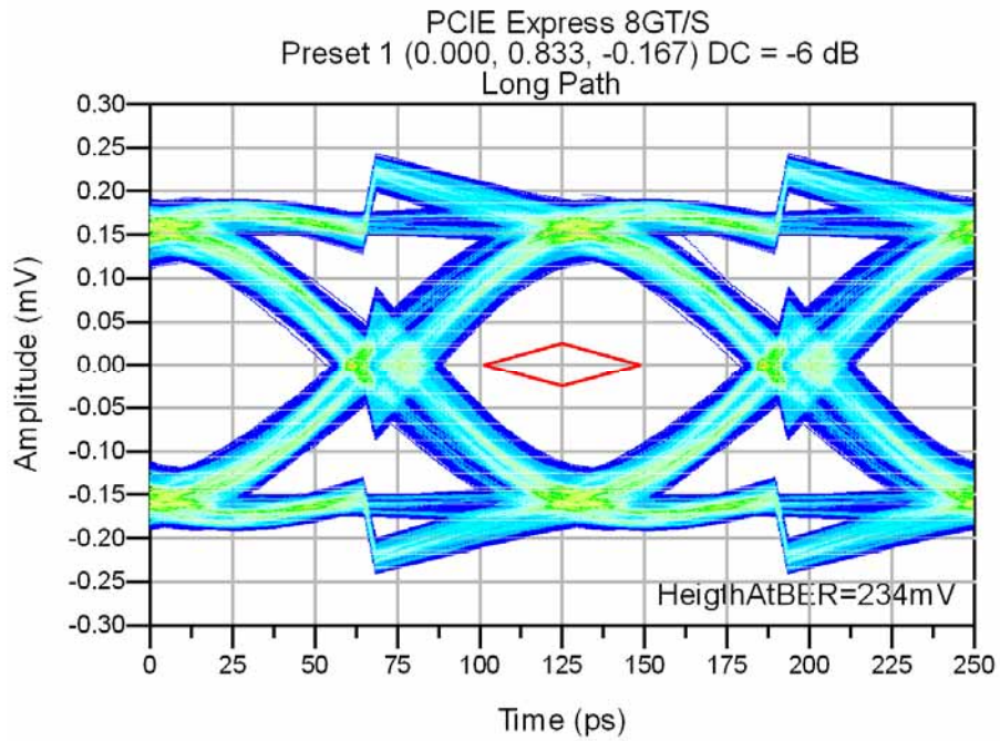
Figure 16 - 8.0 GT/s Eye, Best Case Long Path (0.1" Tx board trace, 0.1" Rx board trace)
