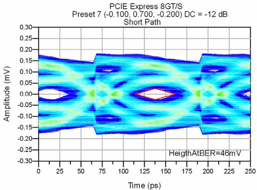
Figure 19 - 8.0 GT/s Eye, Worst Case Short Path (0.6" Tx board trace, 0.8" Rx board trace)
