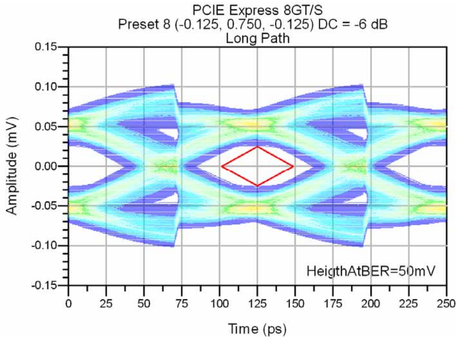
Figure 9 - 100 Ohm System 8.0 GT/s Eye, Long Path (14.0" Tx board trace, 14.0" Rx board trace, with 200 nF DC blocking Capacitor)
