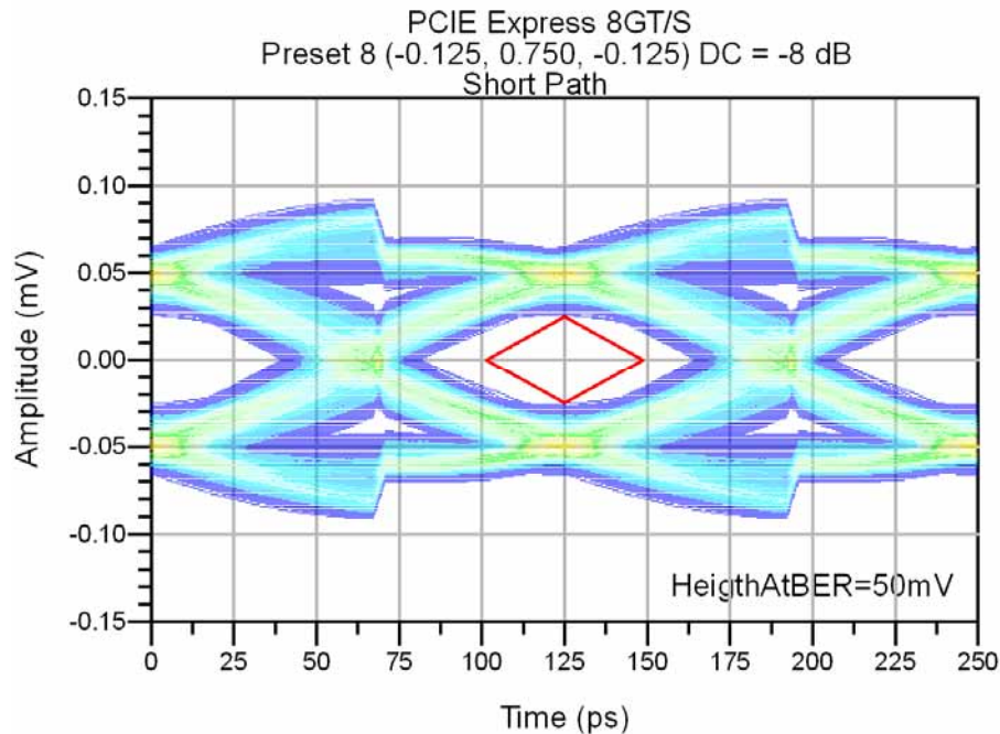
Figure 10 - 100 Ohm System 8.0 GT/s Eye, Short Path (14.5" Tx board trace, 14.5" Rx board trace, with 200 nF DC blocking Capacitor)
