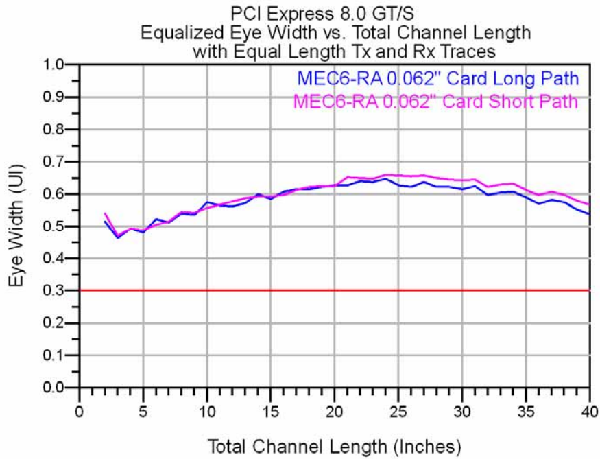
Figure 6 - 100 Ohm System 8.0 GT/s Eye Width vs. Length
