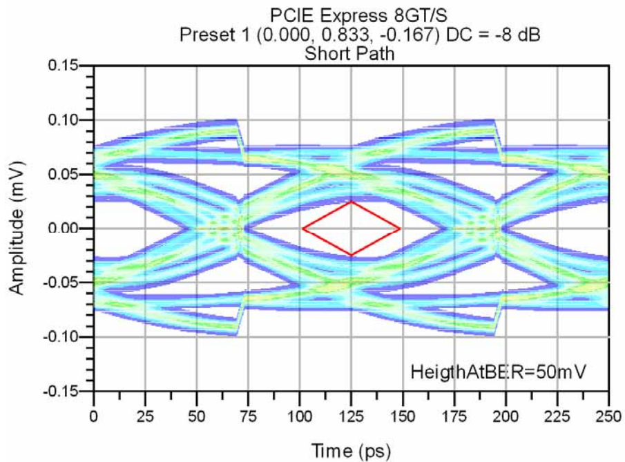
Figure 22 - 85 Ohm System 8.0 GT/s Eye (27.5" Tx board trace, 4" Rx board trace, with 200 nF DC blocking Capacitor)
