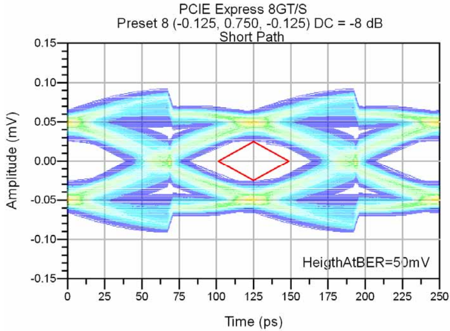
Figure 8 - 100 Ohm System 8.0 GT/s Eye, Short Path (14.5" Tx board trace, 14.5" Rx board trace)
