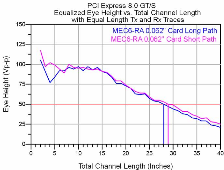
Figure 5 - 100 Ohm System 8.0 GT/s Eye Height vs. Length
