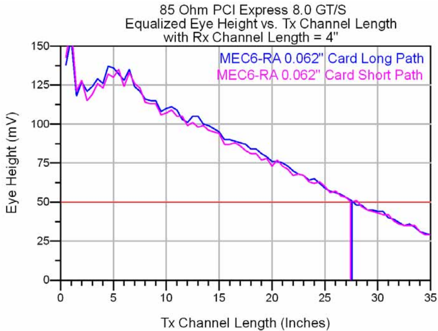
Figure 20 - 85 Ohm System 8.0 GT/s Eye Height vs. Tx Length with Rx Length = 4"
