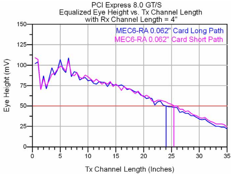
Figure 11 - 100 Ohm System 8.0 GT/s Eye Height vs. Tx Length with Rx Length = 4"
