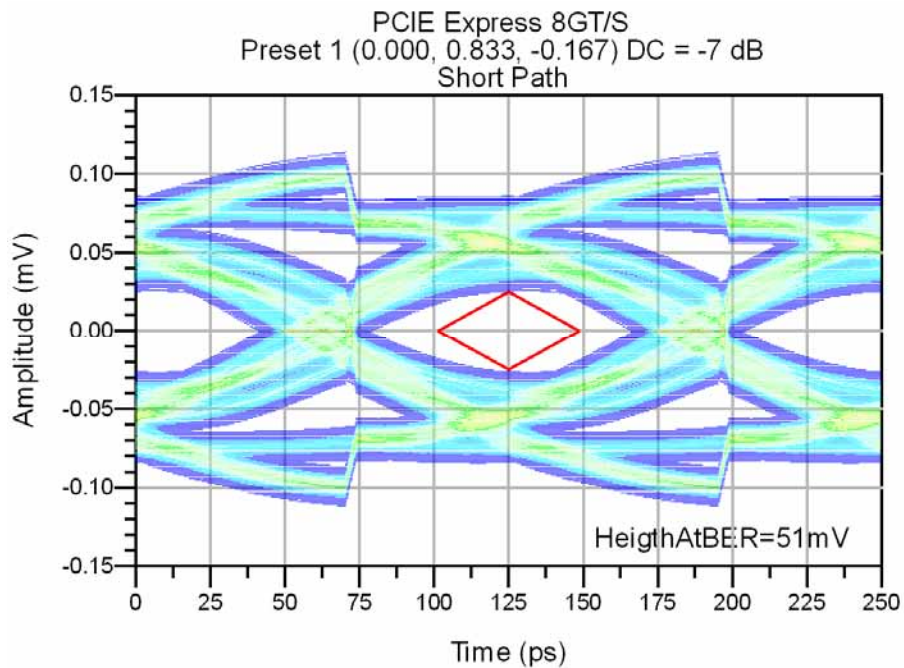
Figure 13 - 8.0 GT/s Eye, Short Path (25" Tx board trace, 4" Rx board trace)
