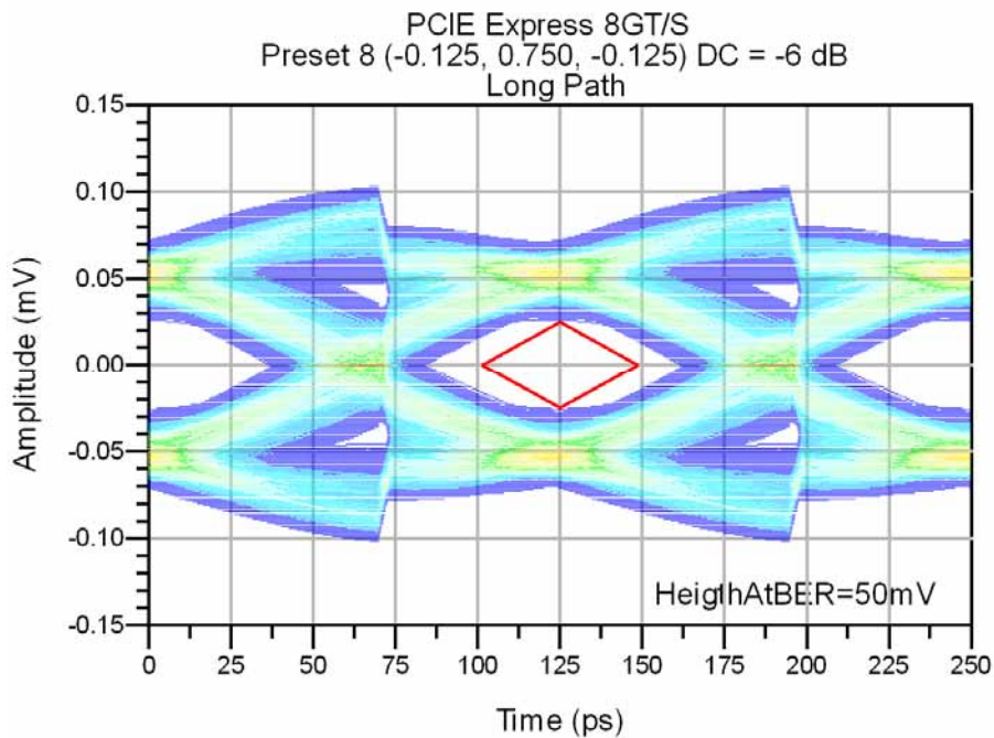
Figure 7 - 100 Ohm System 8.0 GT/s Eye, Long Path (14.0" Tx board trace, 14.0" Rx board trace)
