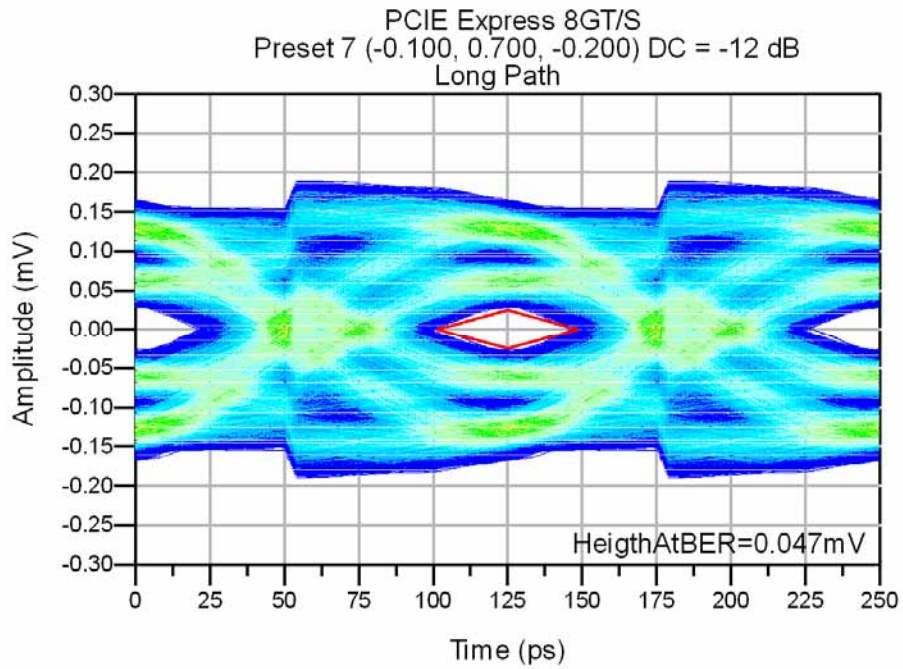
Figure 18 - 8.0 GT/s Eye, Worst Case Long Path (0.6" Tx board trace, 0.6" Rx board trace)
