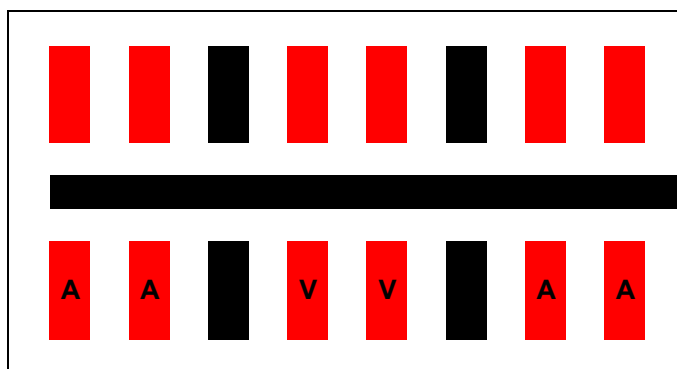
Figure 2 – QTE/QSE single-ended connector pin pattern.
