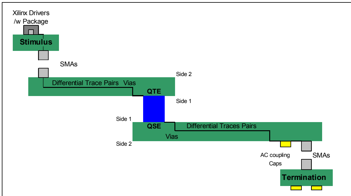
Figure 1 - XAUI Test Circuit
