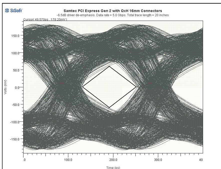
Picture 7 – Receiver eye measurement, probed at far end termination. Standard driver setting with -6.5 dB de-emphasis. Total trace length = 20 inches.
