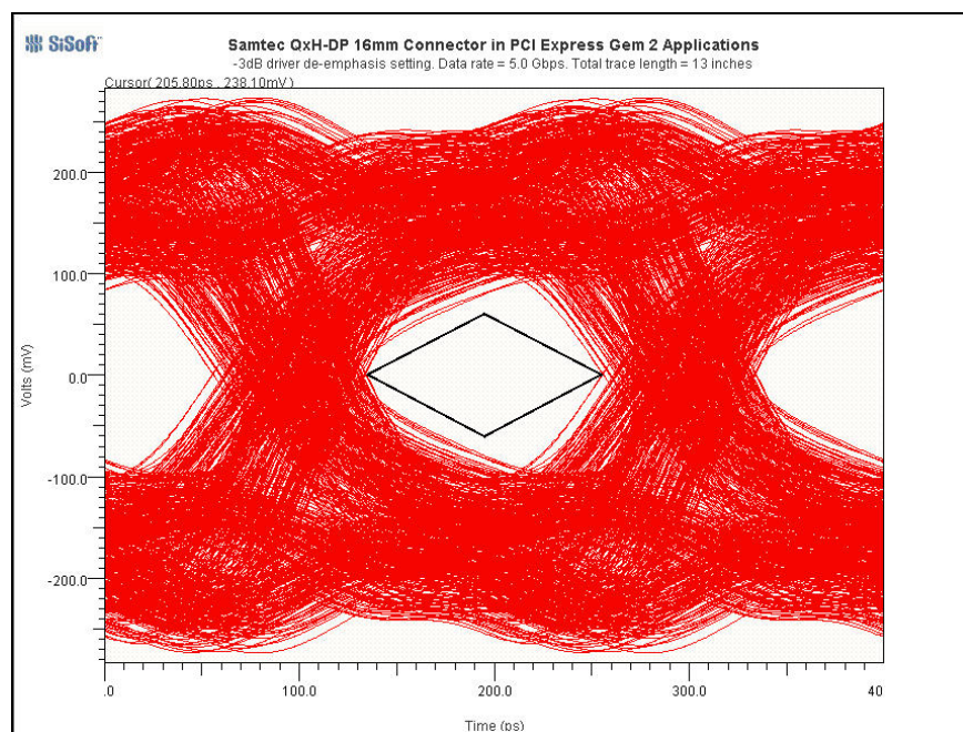
Picture 4 – Receiver eye measurement, probed at far end termination. Normal power driver setting with -3 dB de-emphasis. Total trace length = 13 inches.
