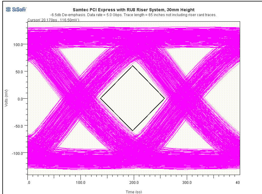
Picture 7 – Receiver eye measurement, probed at far end termination. Standard driver setting with -6.5 dB de-emphasis. Total trace length = 65 inches
