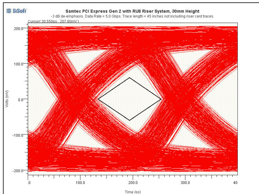
Picture 4 – Receiver eye measurement, probed at far end termination. Normal power driver setting with -3 dB de-emphasis. Total trace length = 45 inches.
