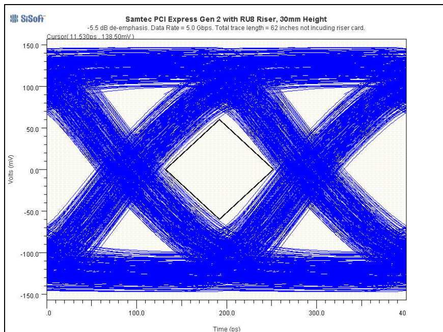
Picture 6 – Receiver eye measurement, probed at far end termination. Normal power driver setting with -5.5 dB de-emphasis. Total trace length = 62 inches
