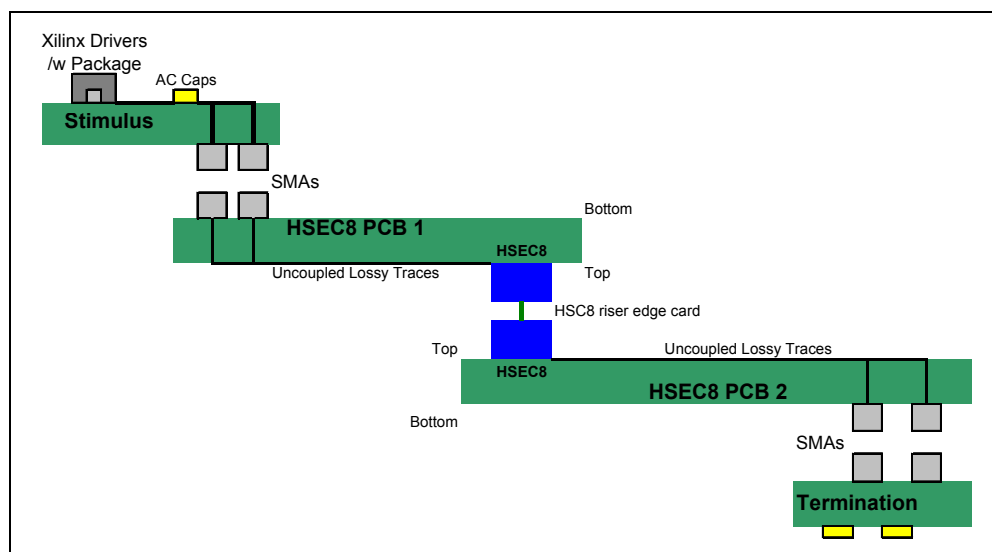
Figure 1 - PCI Express Test Circuit
