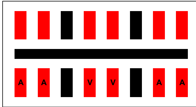
Figure 2 – RU8 differential connector pin pattern. V = Victim pair, A = aggressor pairs, Black = Ground
