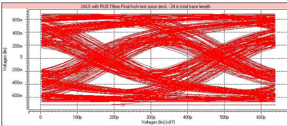
Picture 2 – RiseUp™ RU8 Series XAUI circuit differential eye waveform, probed at terminator pins, 24 inches total trace length.
