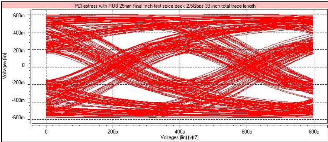
Picture 2 – RiseUp® RU8-DP Series 25mm PCI Express circuit eye waveform, probed at terminator pins, 39 inches total trace length
