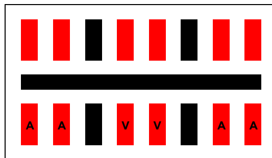
Figure 2 – RiseUp® RU8-DP Series differential connector pin pattern
