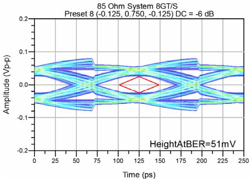
Figure 15 - 85 Ohm System 8.0 GT/s Eye (30" Tx board trace, 4" Rx board trace, with 200 nF DC blocking Capacitor)
