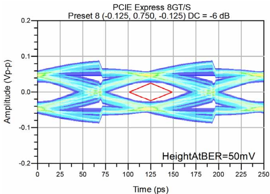
Figure 8 - System 8.0 GT/s Eye (16.75" Tx board trace, 16.75" Rx board trace, with 200 nF DC blocking Capacitor)
