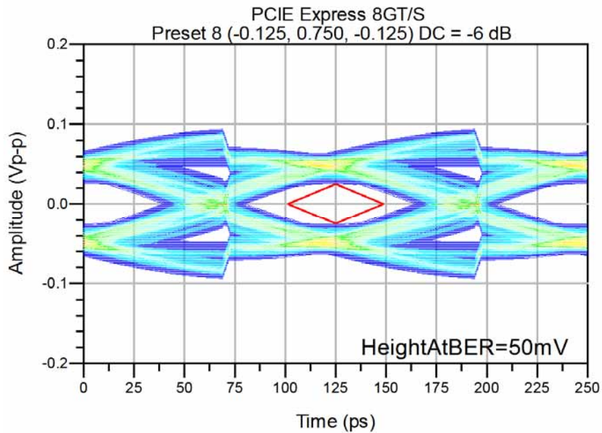
Figure 7 - System 8.0 GT/s Eye (16.75" Tx board trace, 16.75" Rx board trace)
