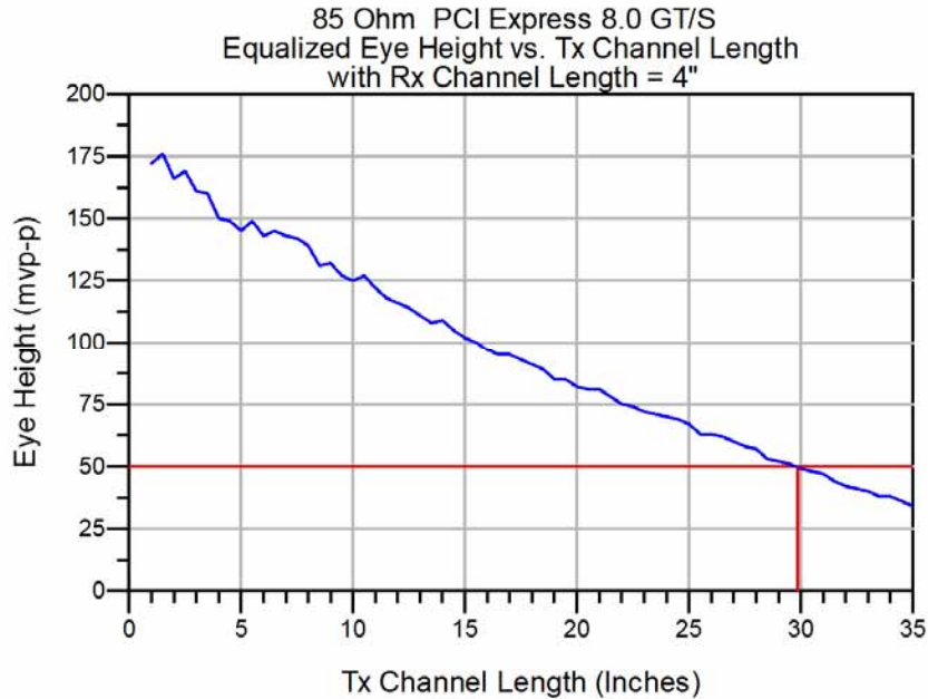
Figure 14 - 85 Ohm System 8.0 GT/s Eye Height vs. Tx Length with Rx Length = 4"
