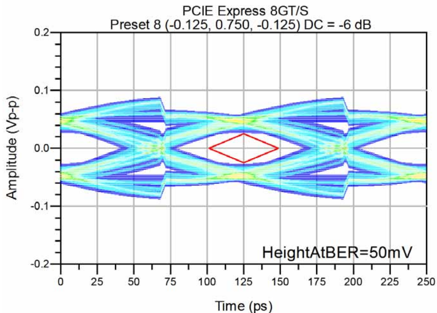
Figure 11 - 8.0 GT/s Eye (29.5" Tx board trace, 4" Rx board trace, with 200 nF DC blocking Capacitor)
