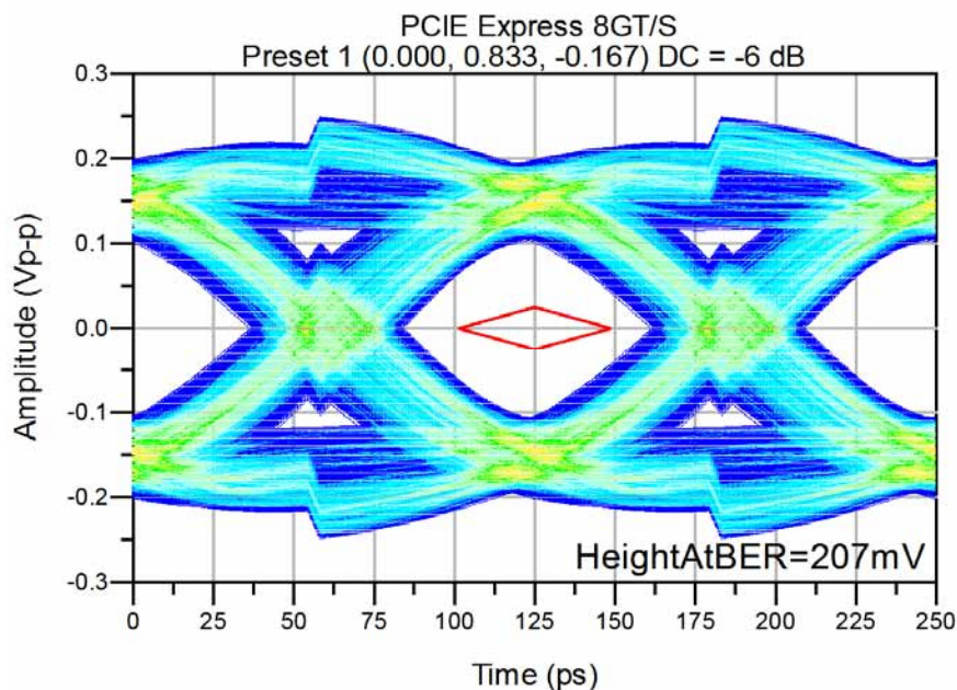
Figure 12 - 8.0 GT/s Eye (0.2" Tx board trace, 0.1" Rx board trace)
