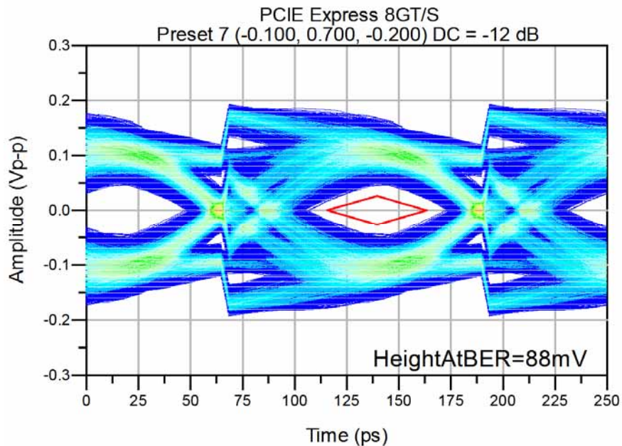
Figure 13 - 8.0 GT/s Eye (0.7" Tx board trace, 0.8" Rx board trace)
