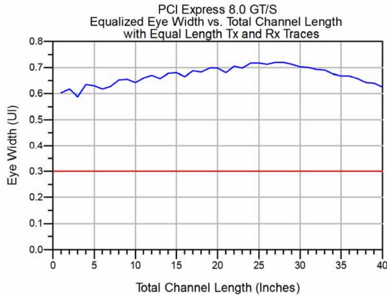
Figure 6 - 8.0 GT/s Eye Width vs. Length
