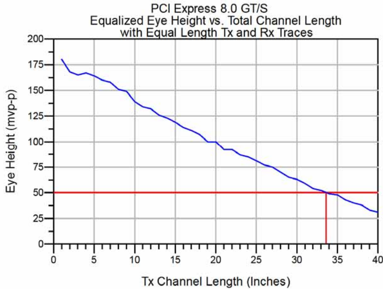
Figure 5 - 8.0 GT/s Eye Height vs. Length
