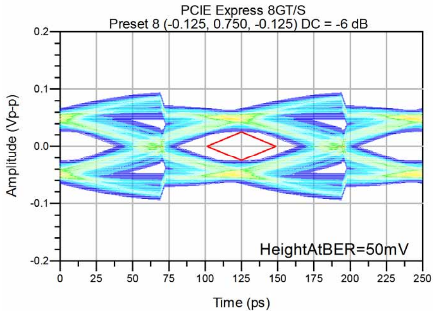
Figure 10 - 8.0 GT/s Eye (29.5" Tx board trace, 4" Rx board trace)
