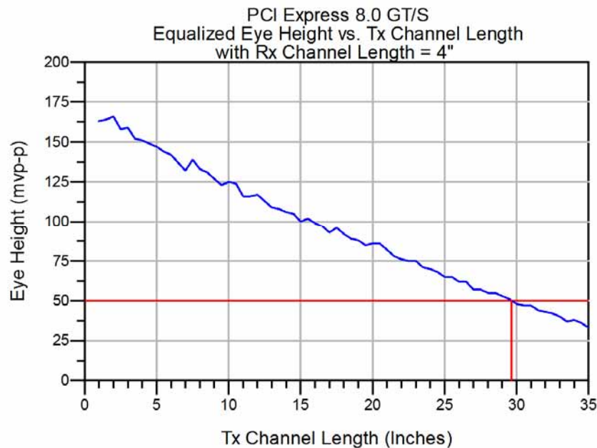
Figure 9 - 8.0 GT/s Eye Height vs. Tx Length with Rx Length = 4"
