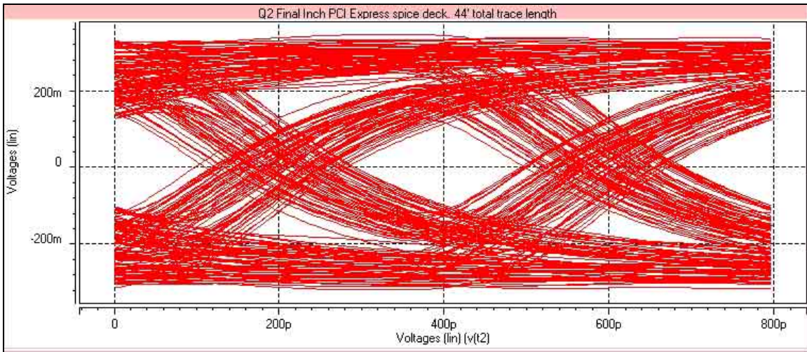
Picture 2 – PCI Express circuit eye waveform, probed at terminator pins, 44 inches total trace length
