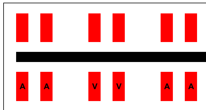
Figure 2 – QMS-DP/QFS-DP Series differential connector pin pattern; V = Victim, A = Aggressor
