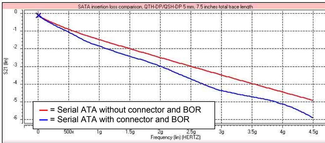
Figure 4 - Insertion loss comparison of 7.5 inch trace with and without connector and breakout
