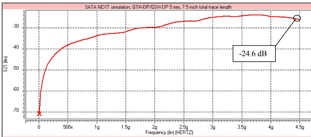
Figure 5 – QTH-DP/QSH-DP 5mm circuit NEXT simulation results, 7.5 inches total trace length
