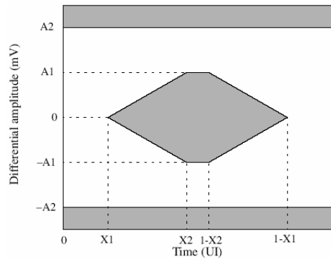
Figure 12 -Example mask template
