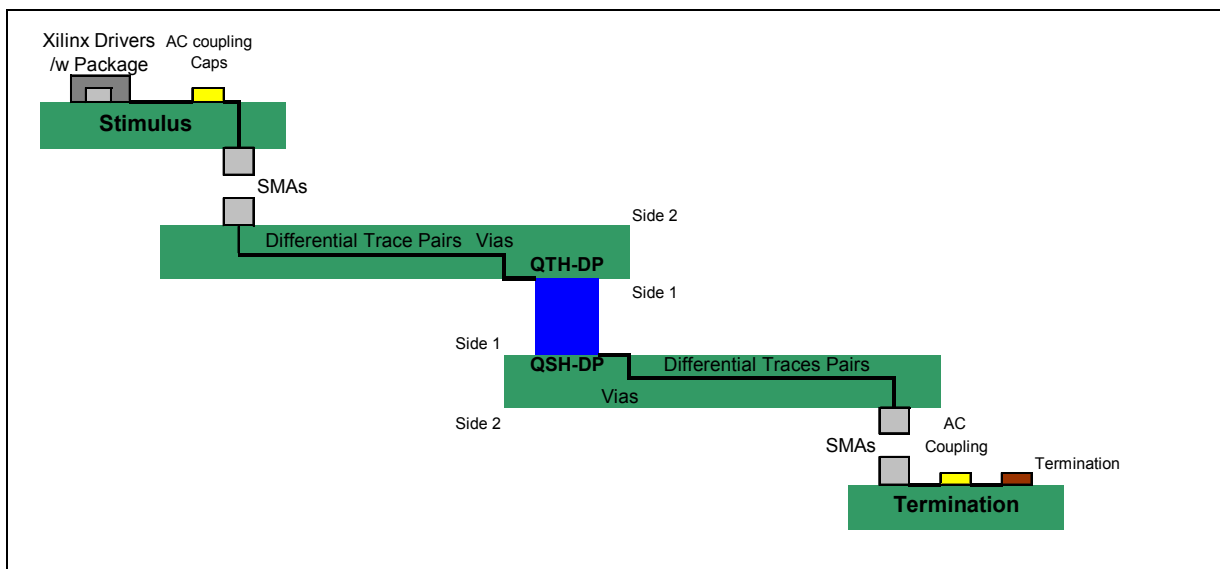
Figure 11 Serial ATA System Test Circuit
