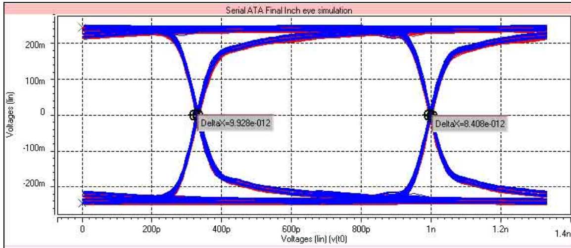
Figure 10 – QTH-DP/QSH-DP Final Inch® circuit eye
