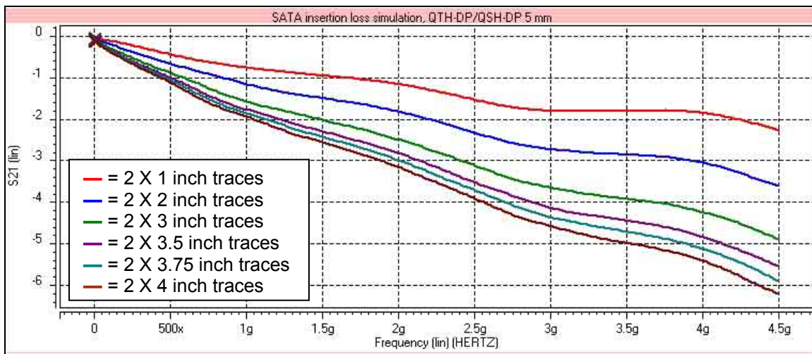
Figure 3 – Serial ATA circuit insertion loss
