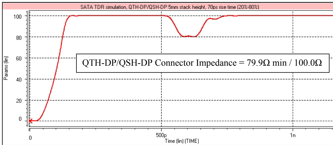
Figure 6 – QTH-DP/QSH-DP 5mm Connector TDR results
