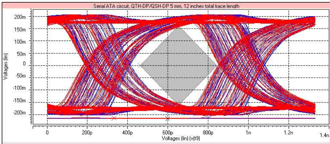
Picture 2 – Serial ATA circuit eye waveform, probed at terminator pins, 12 inches total trace length. Red = circuit with QTH-DP/QSH-DP connector, Blue = circuit without QTH-DP/QSH-DP connector.
