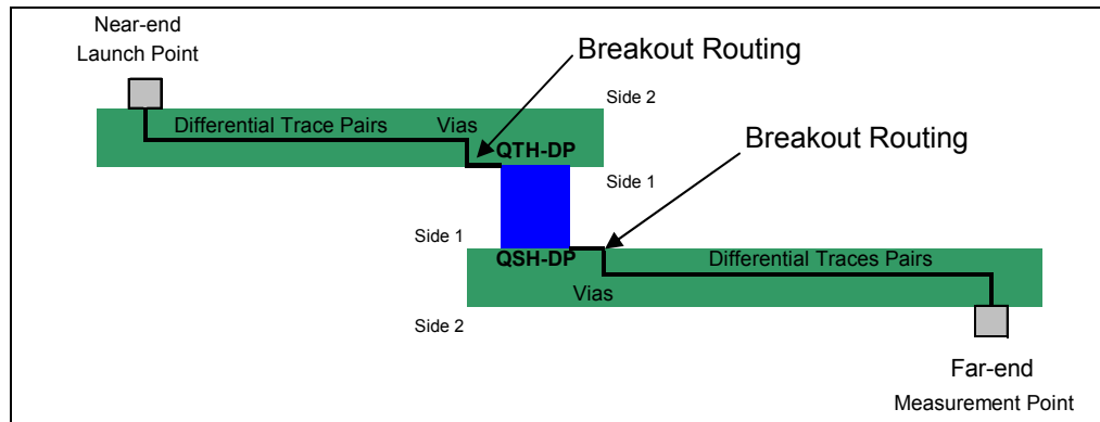
Figure 1 QTH-DP/QSH-DP QPairs® Final Inch® Test Fixture
