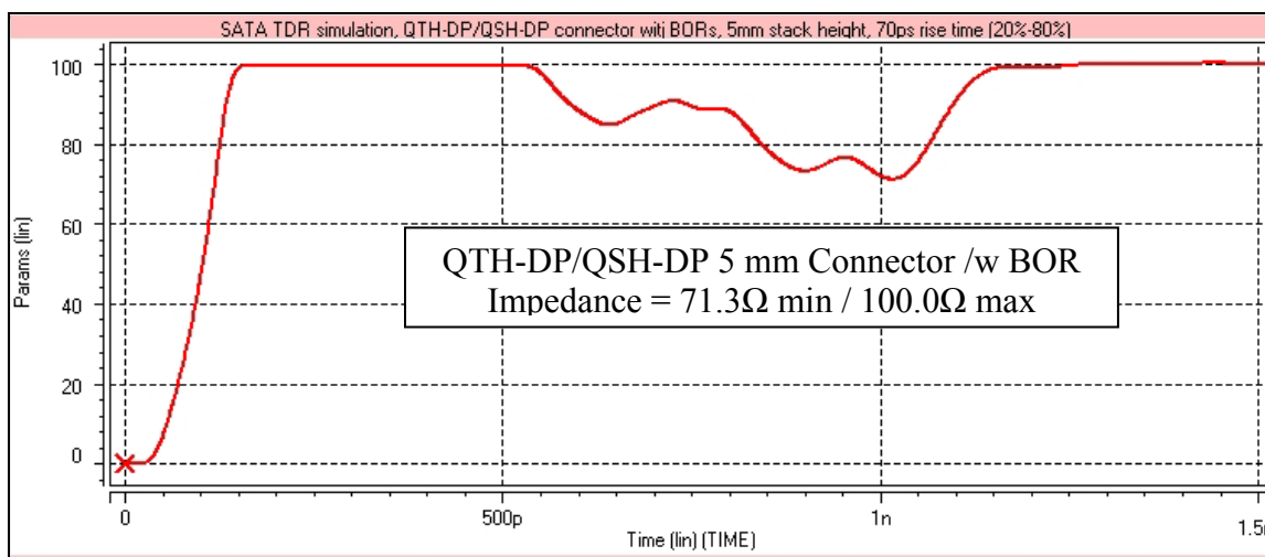
Figure 7 – QTH-DP/QSH-DP Connector with Breakout Routing TDR results
