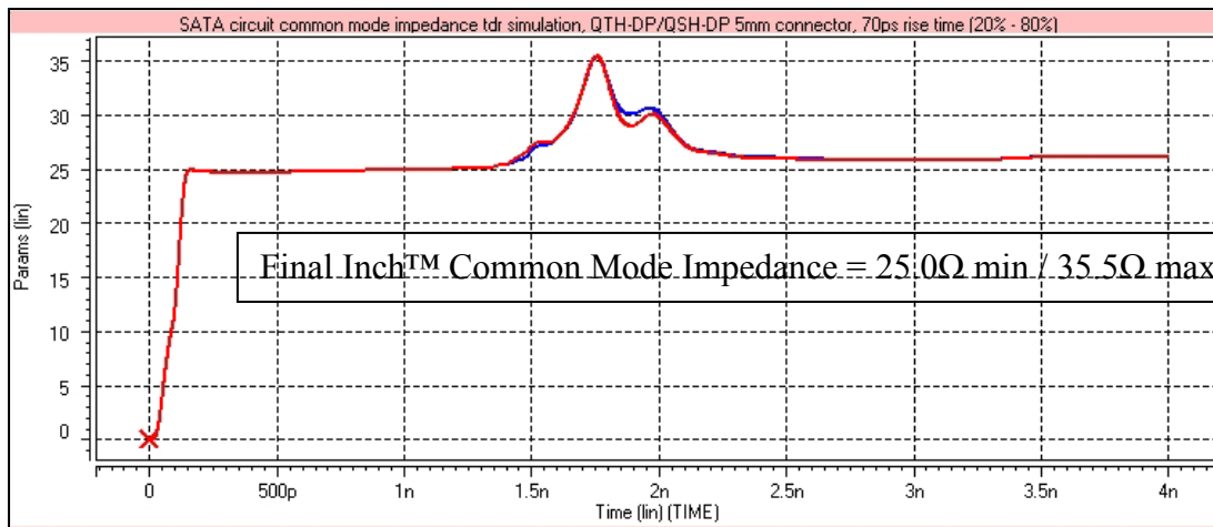
Figure 8 – QTH-DP/QSH-DP Final Inch® Circuit Common Mode Impedance
