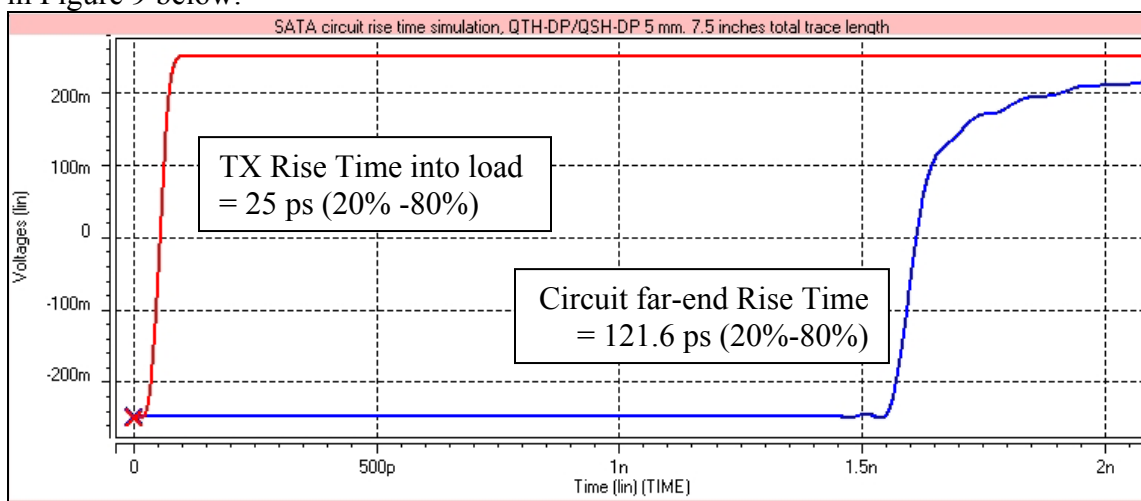
Figure 9 – QTH-DP/QSH-DP Final Inch® circuit rise time results with 7.5 inches total trace length. Red = TX driving compliance load. Blue = Final Inch® circuit probed at the far-end termination.
