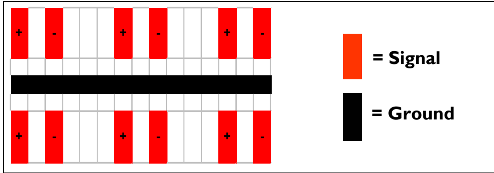
Figure 2 - QTH-DP/QSH-DP differential connector pin pattern
