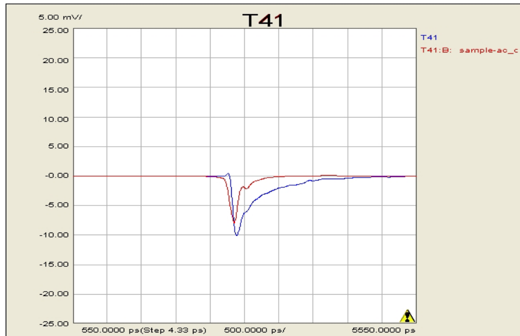
Figure 9: Measured and Simulated Far End Crosstalk - Short Path
