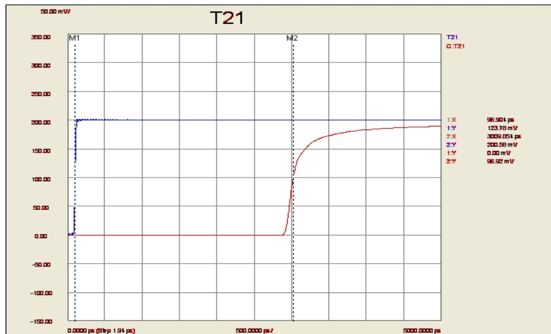
Figure 5: Measured Propagation Delay Long Path.
