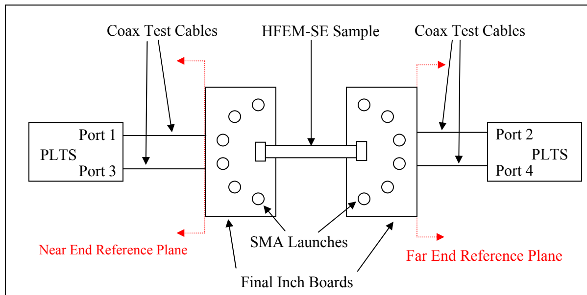
Figure 20: Measurement Setup.
