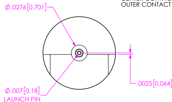
DETAIL 'A' SCALE 10 : 1
