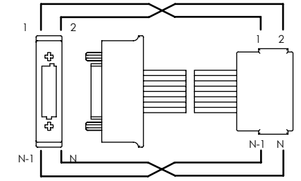
WIRING OPTION 1 POSITION 1 TO POSITION 1
