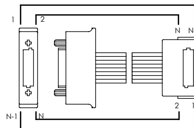
WIRING OPTION 3 POSITION 1 TO POSITION N-1
