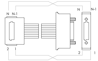
WIRING OPTION 1 POSITION 1 TO POSITION 1
