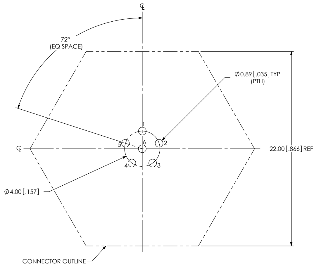
FIG 5 ACRK-12-03-X-T-BT-X-X SHOWN
