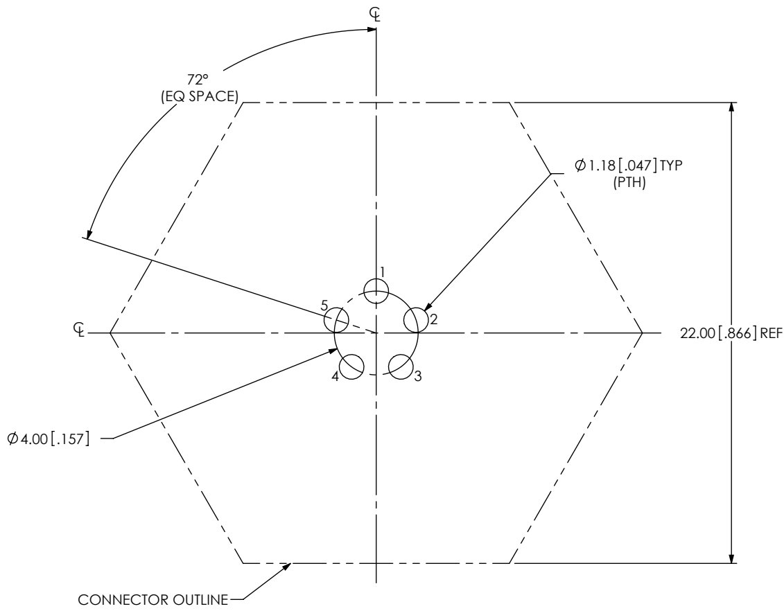
FIG 3 ACRK-12-02-X-T-BT-X-X SHOWN
