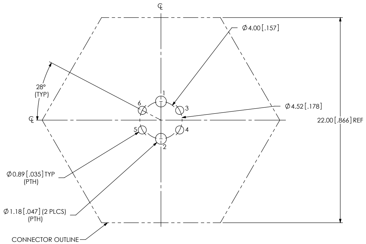
FIG 9 ACRK-12-05-X-T-BT-X-X SHOWN
