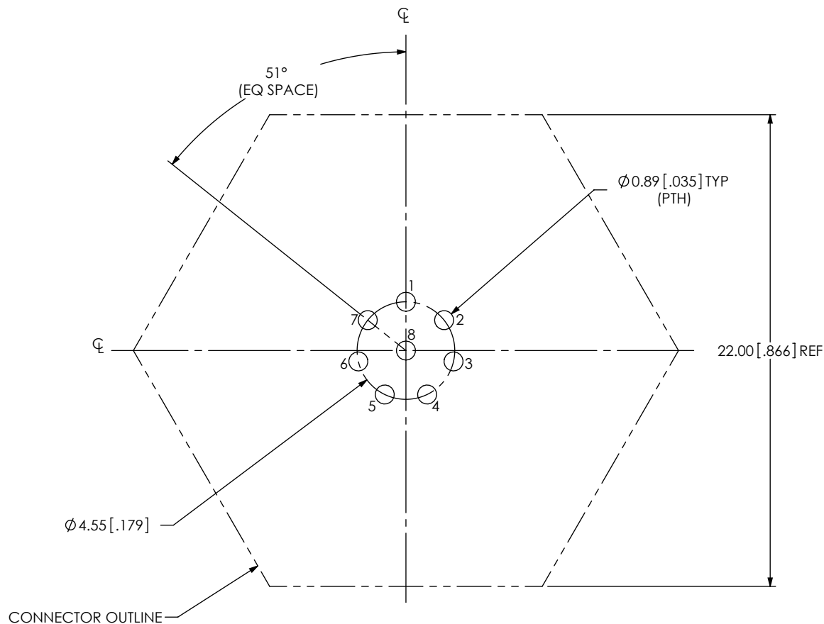
FIG 7 ACRK-12-04-X-T-BT-X-X SHOWN
