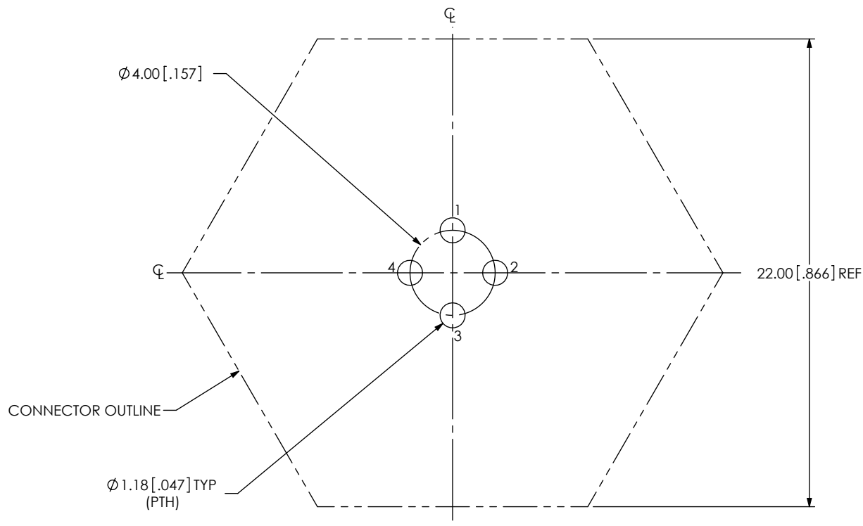
FIG 1 ACRK-12-01-X-T-BT-X-X SHOWN ALL DIMENSIONS ARE SYMMETRIC ABOUT THE CENTERLINE.
