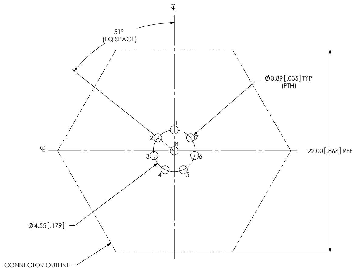
FIG 8 ACRK-12-04-X-S-BT-X-X SHOWN
