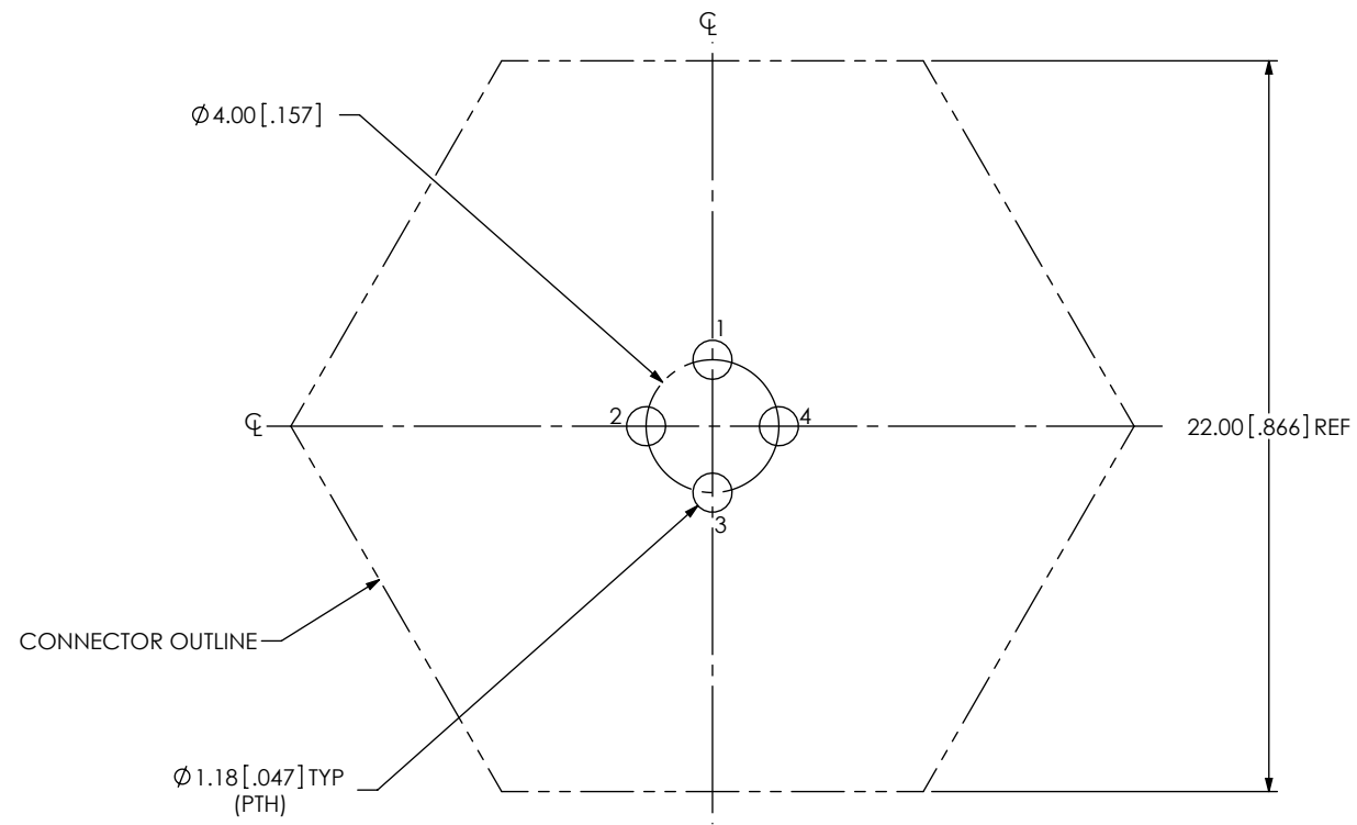
FIG 2 ACRK-12-01-X-S-B1-X-X SHOWN
