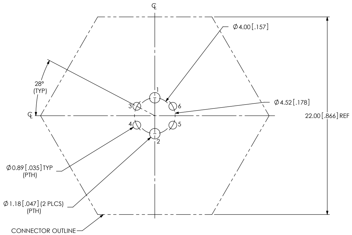
FIG 10 ACRK-12-05-X-S-B1-X-X SHOWN
