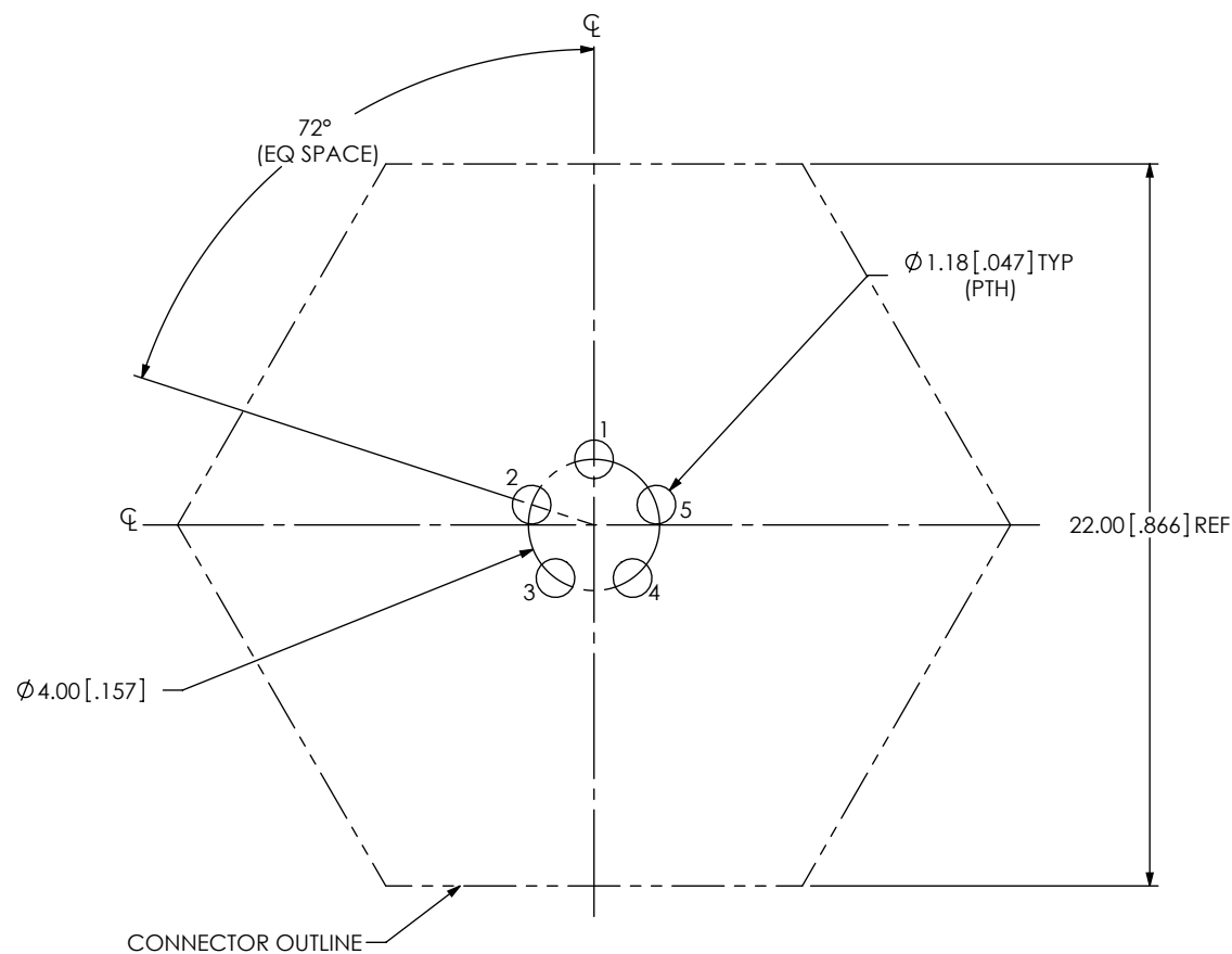
FIG 4 ACRK-12-02-X-S-BT-X-X SHOWN
