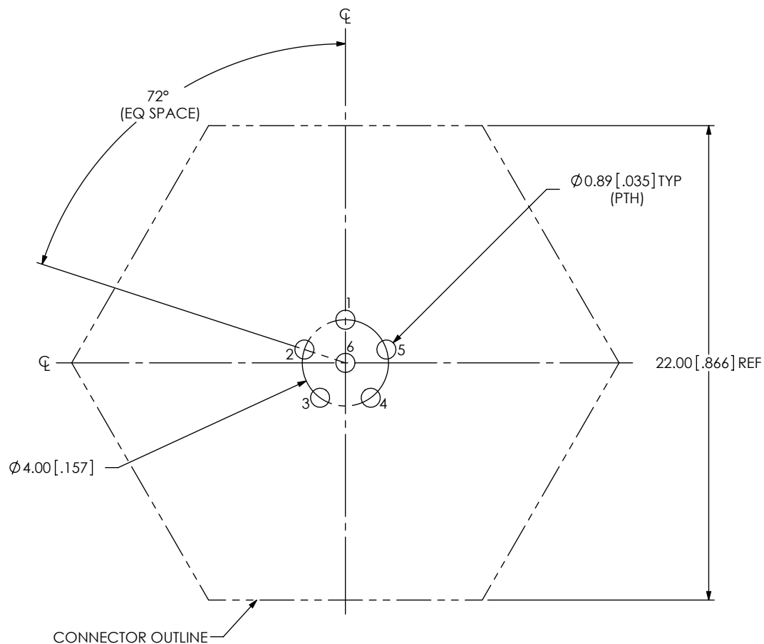
FIG 6 ACRK-12-03-X-S-BT-X-X SHOWN
