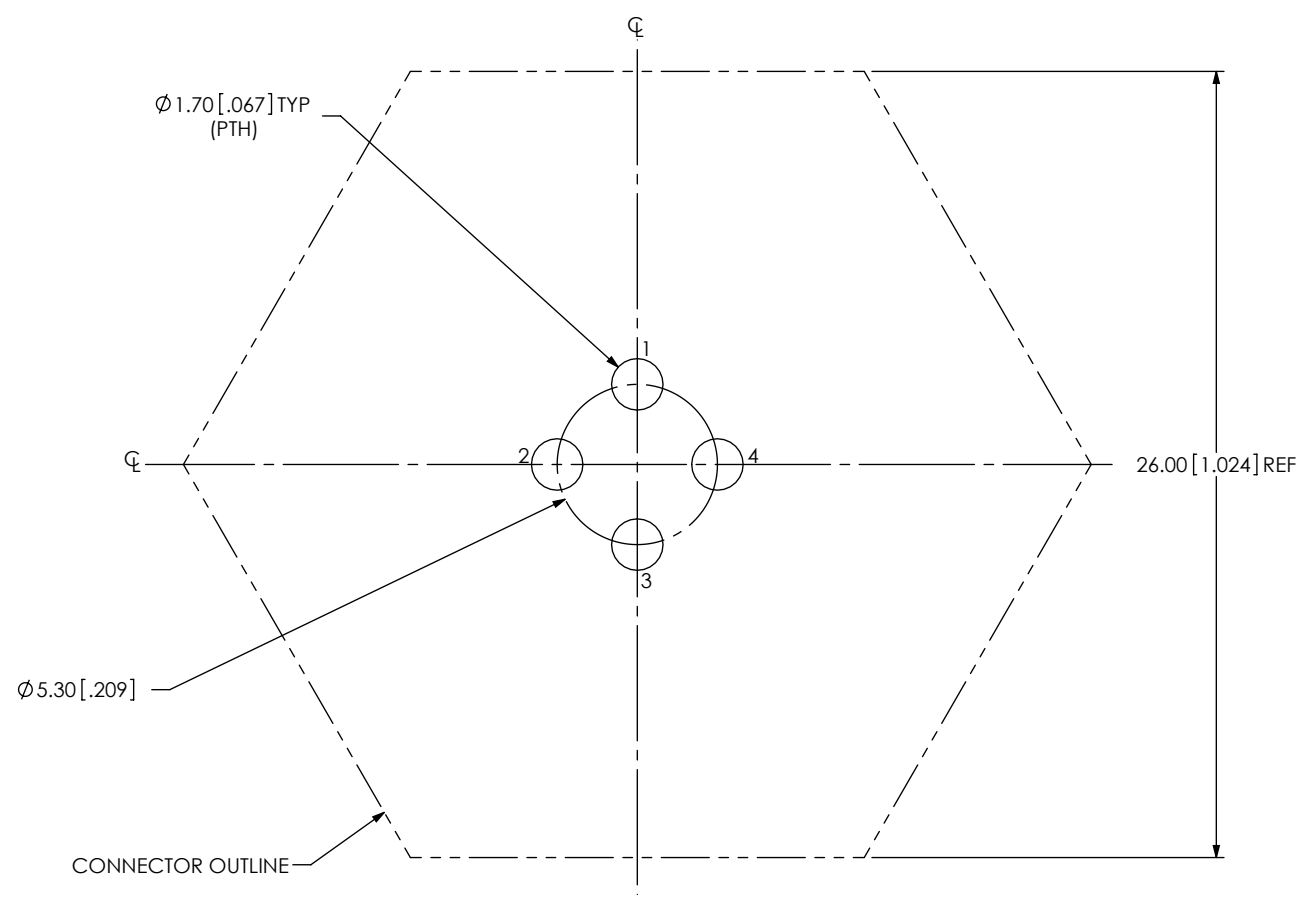
FIG 6 ACRK-16-03-X-S-BT-X-X SHOWN
