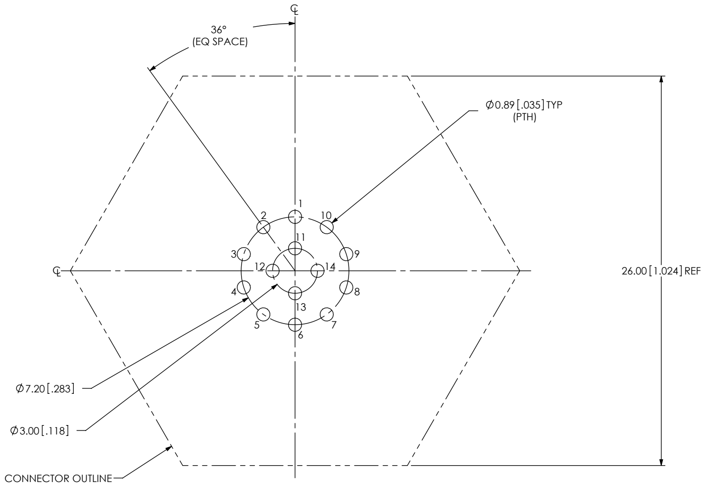
FIG 2 ACRK-16-01-X-S-B1-X-X SHOWN
