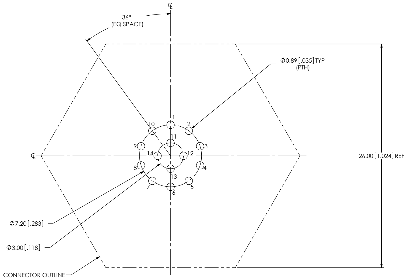
FIG 1 ACRK-16-01-X-T-B1-X-X SHOWN
