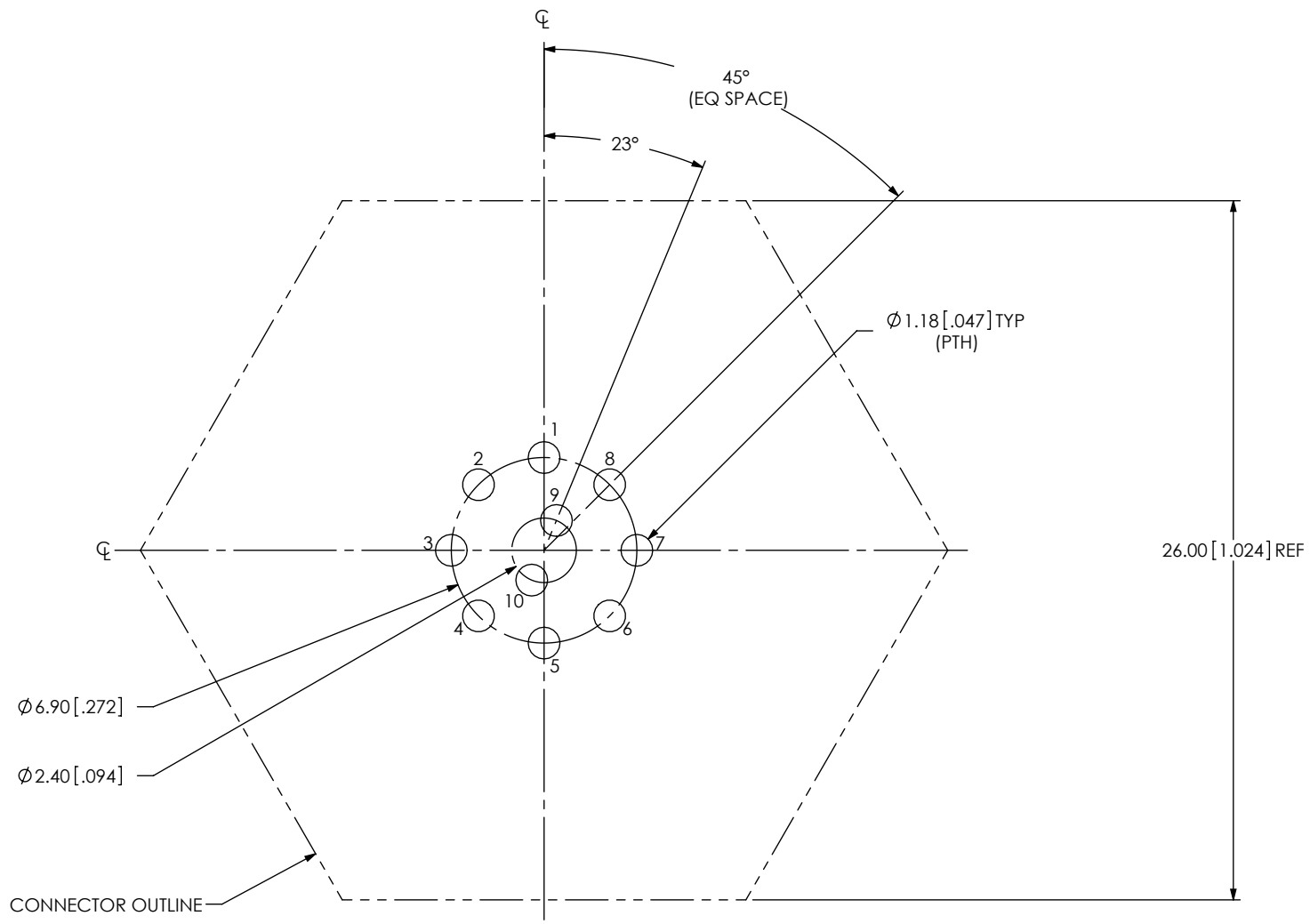
FIG 4 ACRK-16-02-X-S-BT-X-X SHOWN
