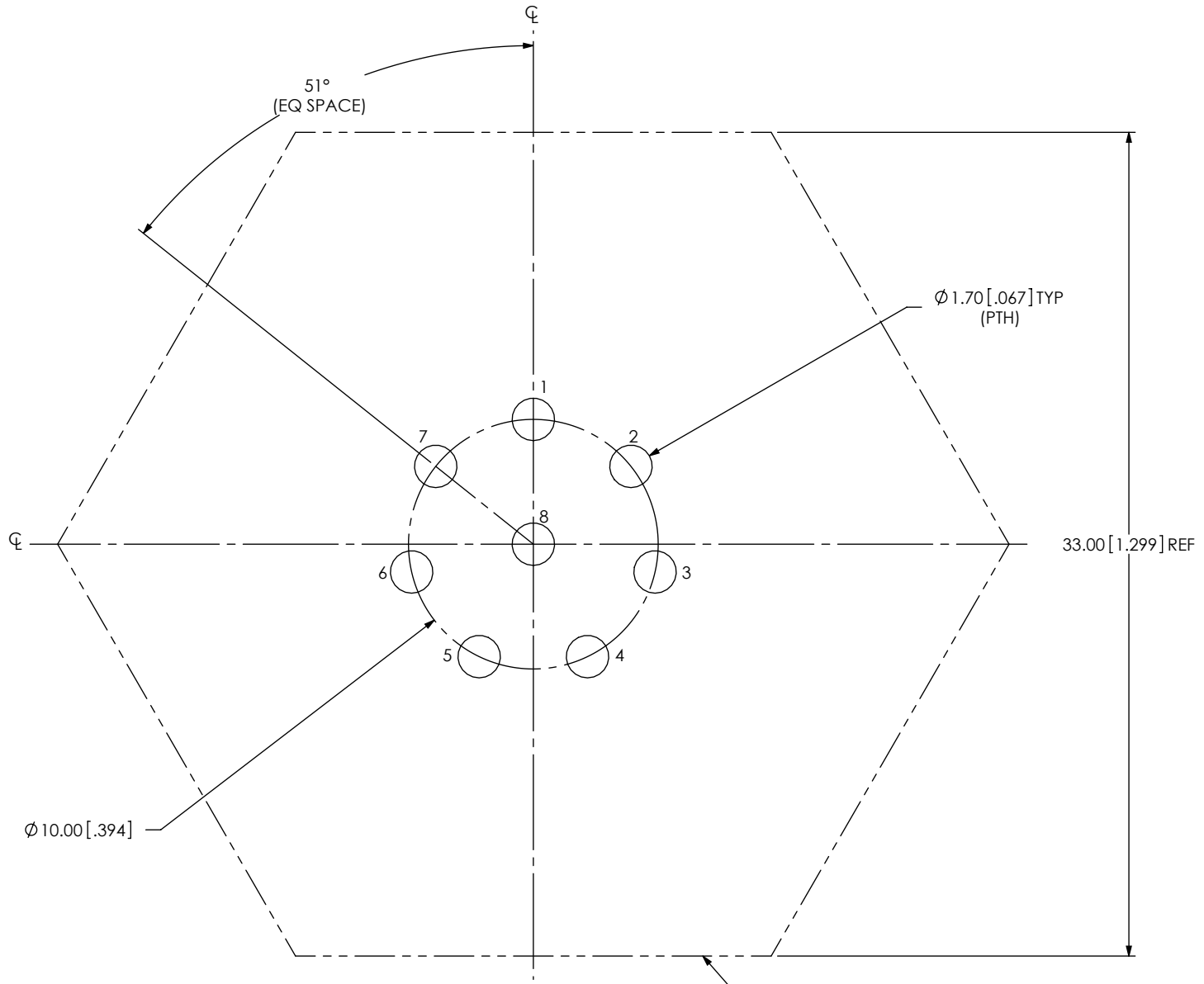
FIG 5 ACRK-22-03-X-T-BT-X-X SHOWN
