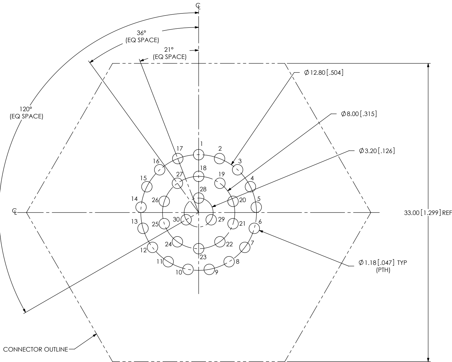
FIG 1 ACRK-22-01-X-T-BT-X-X SHOWN
