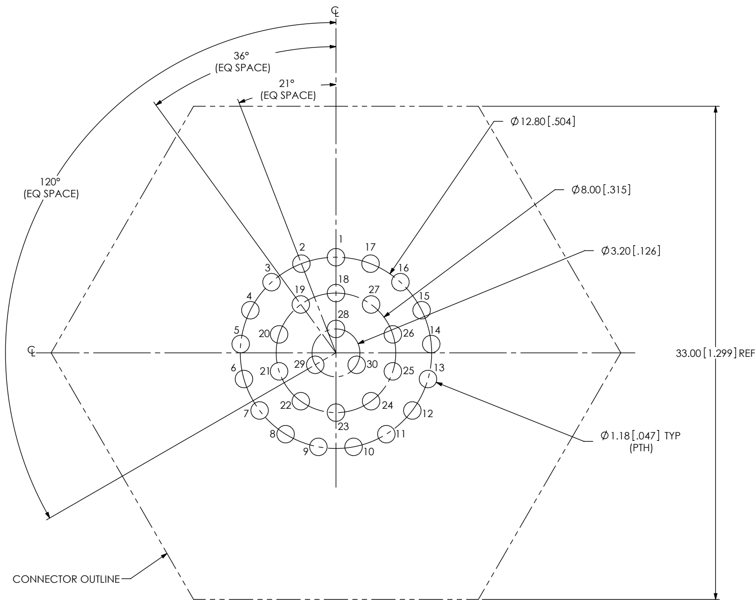
FIG 2 ACRK-22-01-X-S-BT-X-X SHOWN
