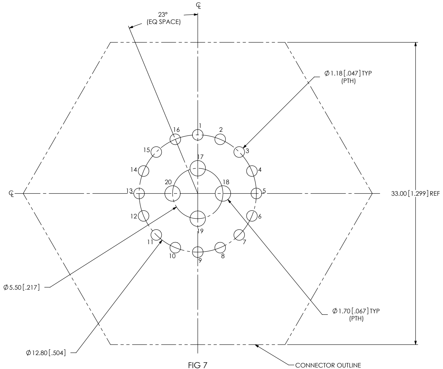
FIG 7 ACRK-22-05-X-T-BT-X-X SHOWN
