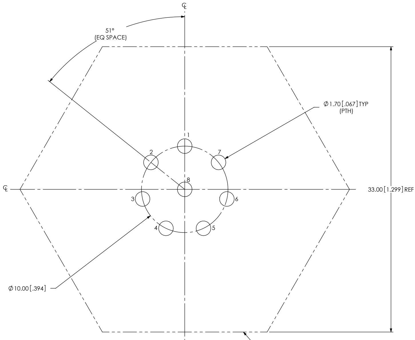
FIG 6 ACRK-22-03-X-S-BT-X-X SHOWN
