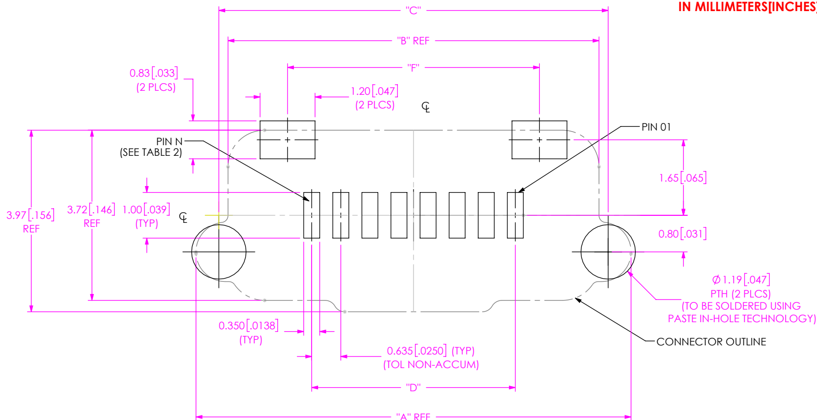
FIG 1 (AMF6-02-X-K-XR FOOTPRINT SHOWN) (ALL DIMENSIONS ARE SYMMETRIC ABOUT THE CENTERLINE)
