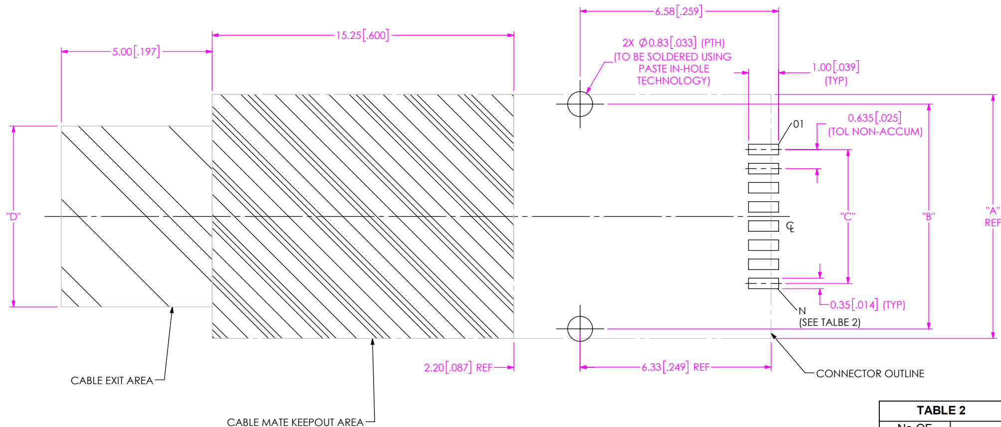
FIG 1 (AMF6-02-S-RA-XR FOOTPRINT SHOWN) (ALL DIMENSIONS ARE SYMMETRIC ABOUT THE CENTERLINE)
