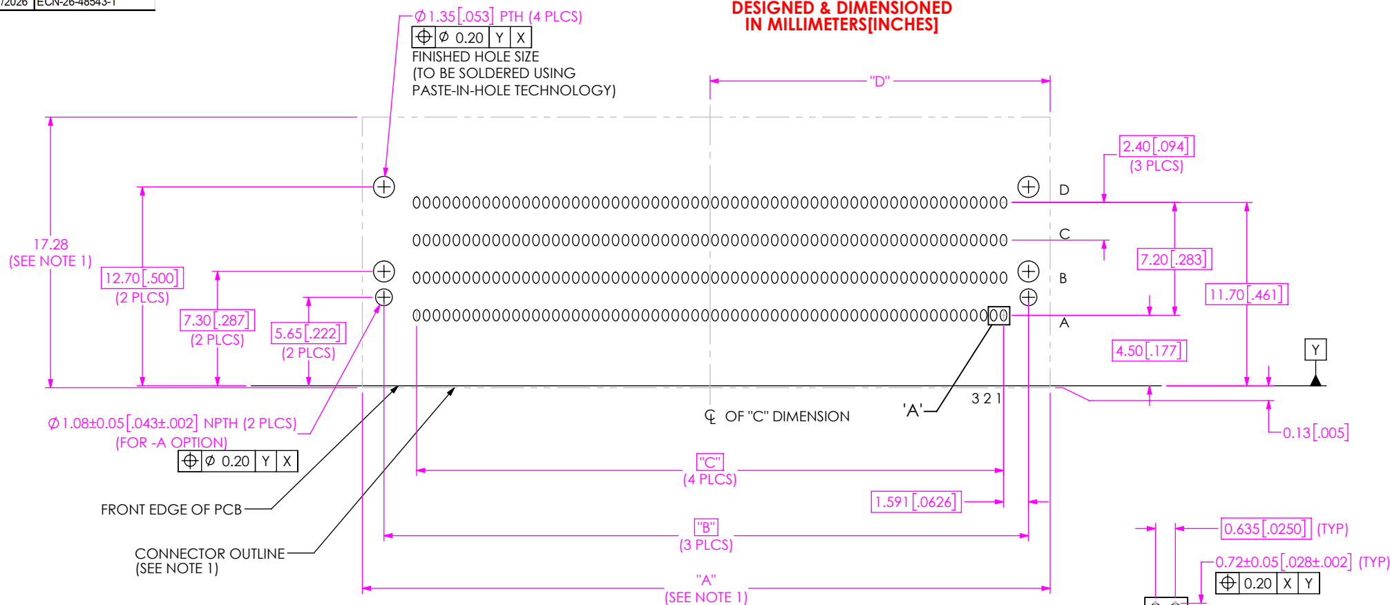
FIG 1 APF6-060-S-04-2-RA FOOTPRINT SHOWN
