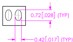
DETAIL 'B' SCALE 8:1 (SURFACE MOUNT PAD)
