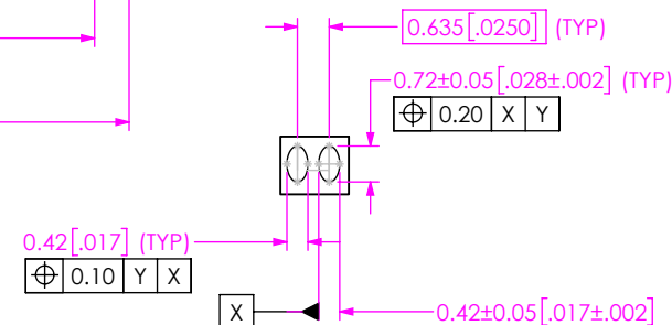
DETAIL 'A' SCALE 6 : 1 (SURFACE MOUNT PAD)
