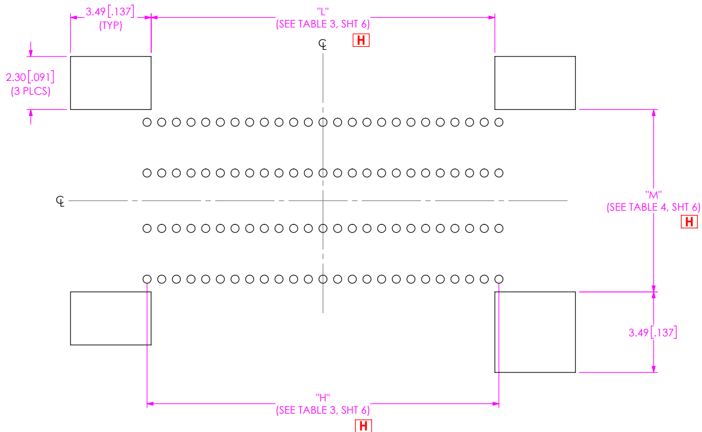
FIG 9 APF6-025-XX.X-XXX-04-2-X STENCIL SHOWN (FOR -L & -T OPTION ONLY) (SAME AS FIG 2, EXCEPT AS SHOWN)
