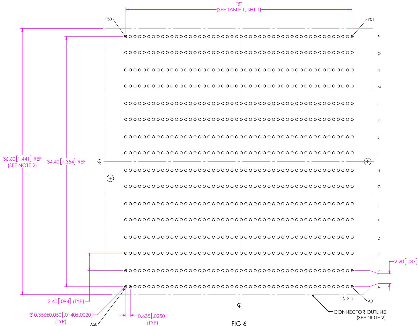
FIG 6 (16 ROW) APF6-050-XX.X-XXX-16-X-A FOOTPRINT SHOWN (SAME AS FIG 1, EXCEPT AS SHOWN)
