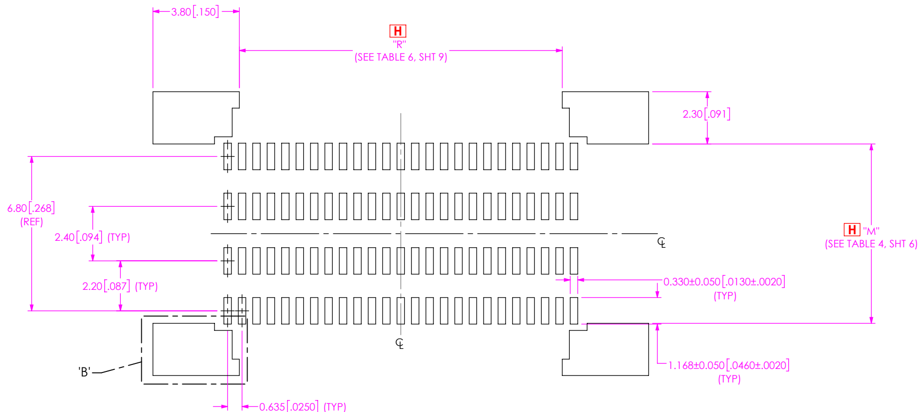
H FIG 16 APF6-025-XX.X-XXX-04-0 STENCIL SHOWN (FOR -0 OPTION ONLY) (FOR -L & -T OPTIONS ONLY) (SAME AS FIG 2, EXCEPT AS SHOWN)
