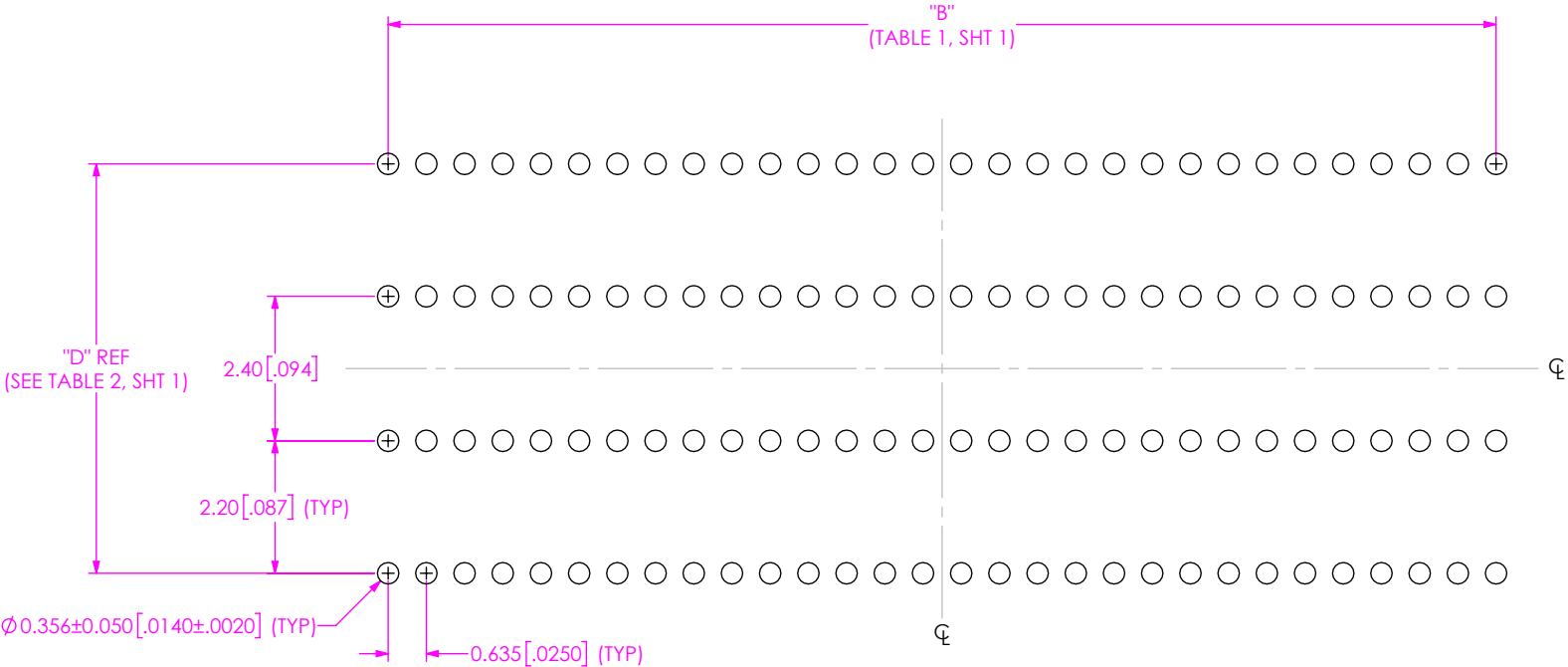
FIG 2 APF6-030-XX.X-XXX-04-2 STENCIL SHOWN
