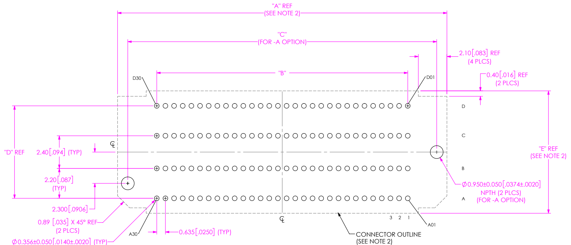
FIG 1 APF6-030-XX.X-XXX-04-X-A FOOTPRINT SHOWN
