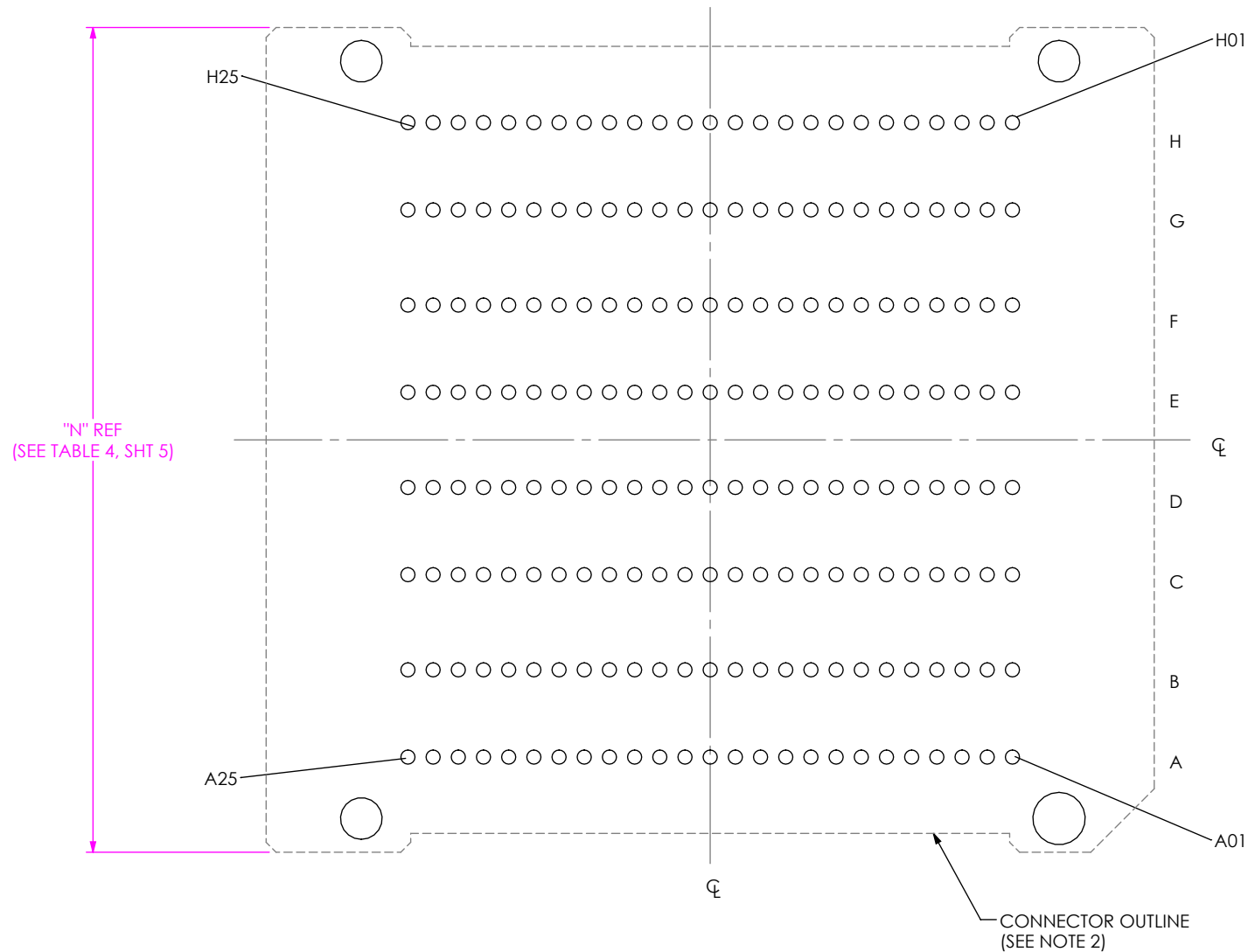
FIG12 APF6-025-XX.X-XXX-08-X-T FOOTPRINT SHOWN (SAME AS FIG 4 & FIG 7, EXCEPT AS SHOWN)
