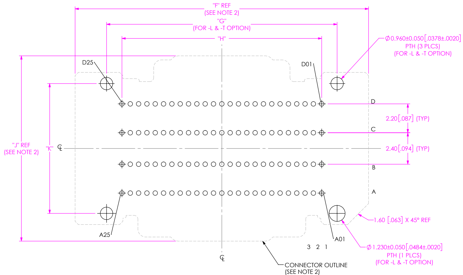
FIG 7 APF6-025-XX.X-XXX-04-X-L FOOTPRINT SHOWN (SAME AS FIG 1, EXCEPT AS SHOWN)
