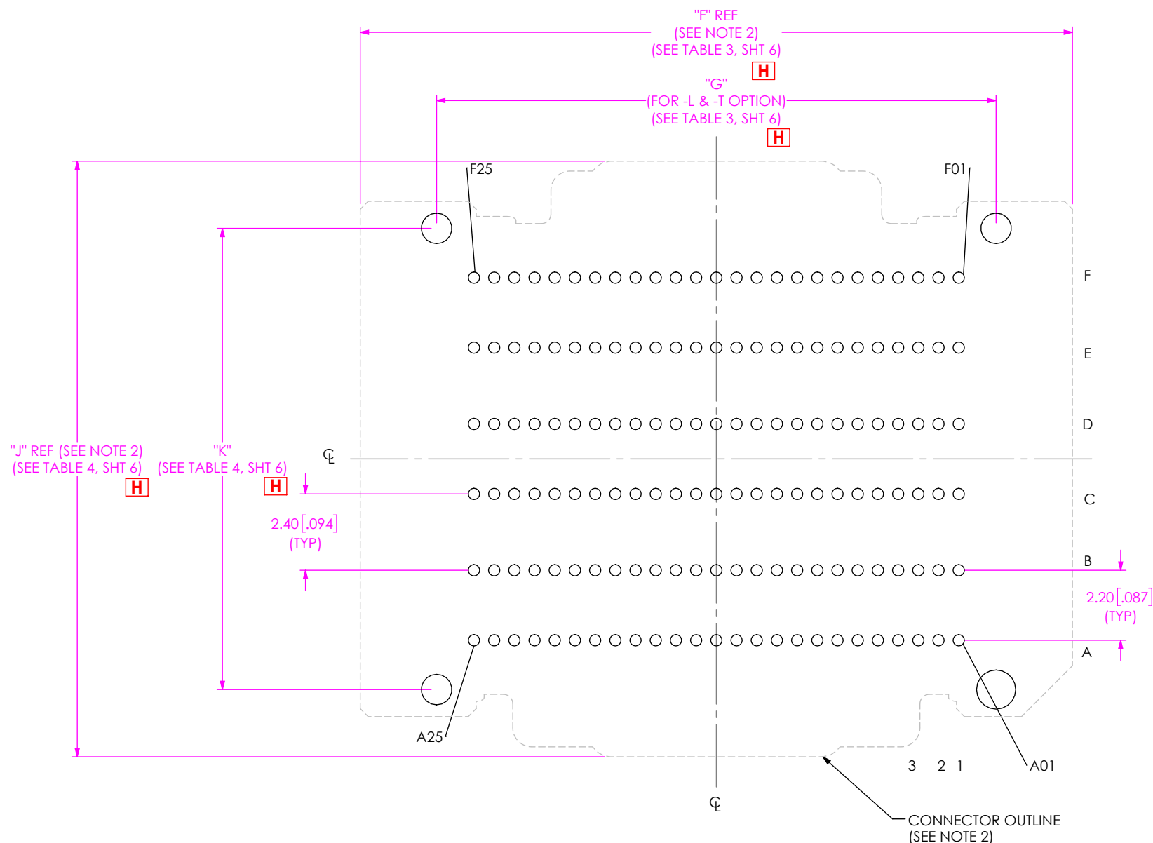
FIG 8 APF6-025-XX.X-XXX-06-X-L FOOTPRINT SHOWN (SAME AS FIG 1, EXCEPT AS SHOWN)
