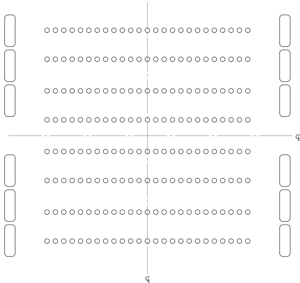
FIG14 APF6-025-XX.X-XXX-08-X-TS STENCIL SHOWN (SAME AS FIG 13, EXCEPT AS SHOWN)
