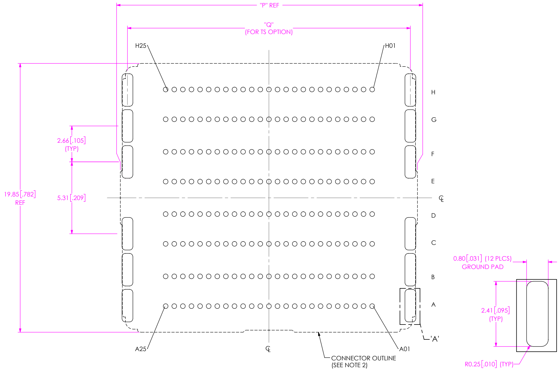
FIG13 APF6-025-XX.X-XXX-08-X-TS FOOTPRINT SHOWN (SAME AS FIG 4, EXCEPT AS SHOWN)
