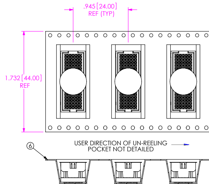
PACKAGING VIEW SCALE 1:1
