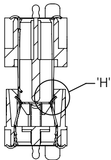
SECTION "E"-"E"
