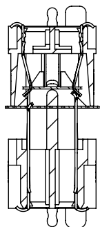
SECTION "F"-"F"
