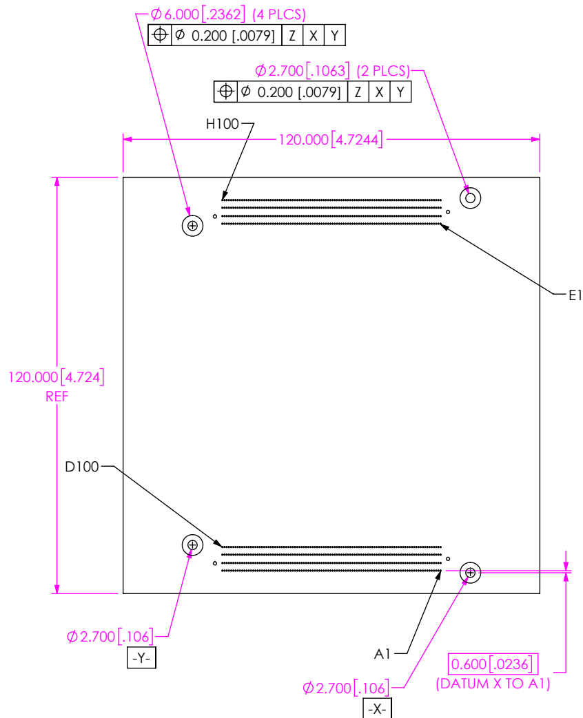
FIG 3 COM-HPC® MODULE SIZE B (SAME AS FIG 2, EXCEPT AS SHOWN) (RECOMMENDED PCB LAYOUT FOR COM-HPC)
