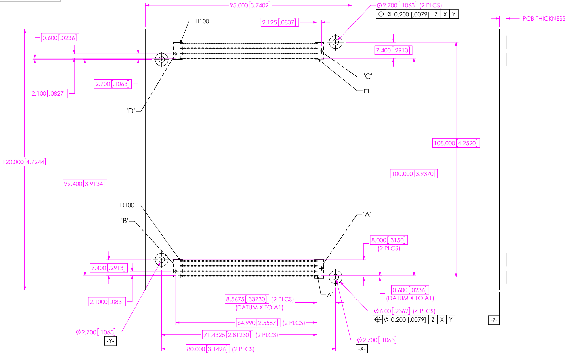
FIG 2 COM-HPC® MODULE SIZE A ((RECOMMENDED PCB LAYOUT FOR COM-HPC®))
