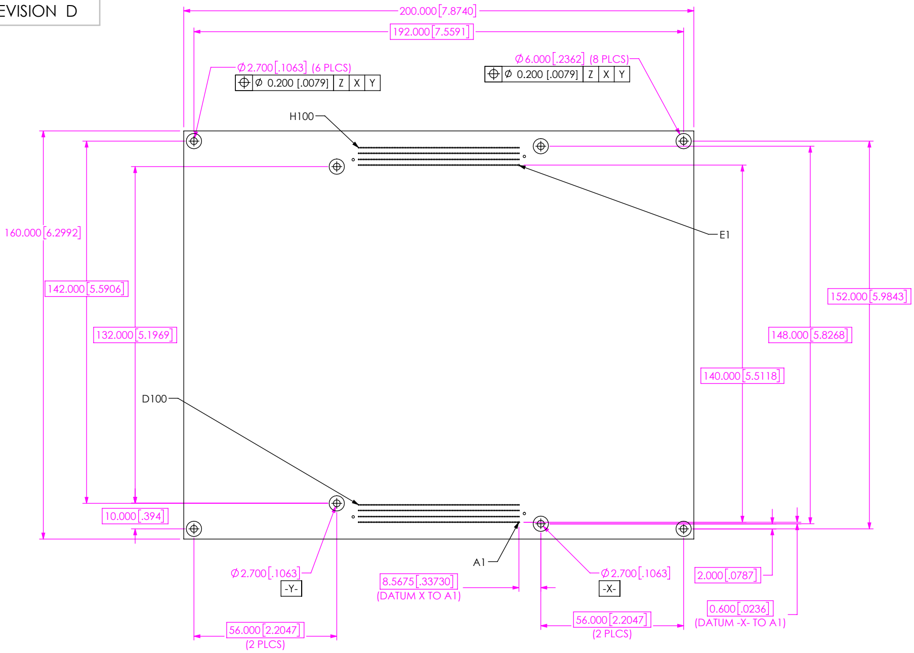
FIG 6 COM-HPC® MODULE SIZE E (SAME AS FIG 2, EXCEPT AS SHOWN) (RECOMMENDED PCB LAYOUT FOR COM-HPC®)
