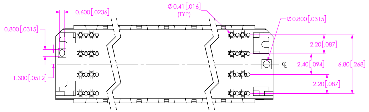
FIG 1 (ASP-209946-02 SHOWN)
