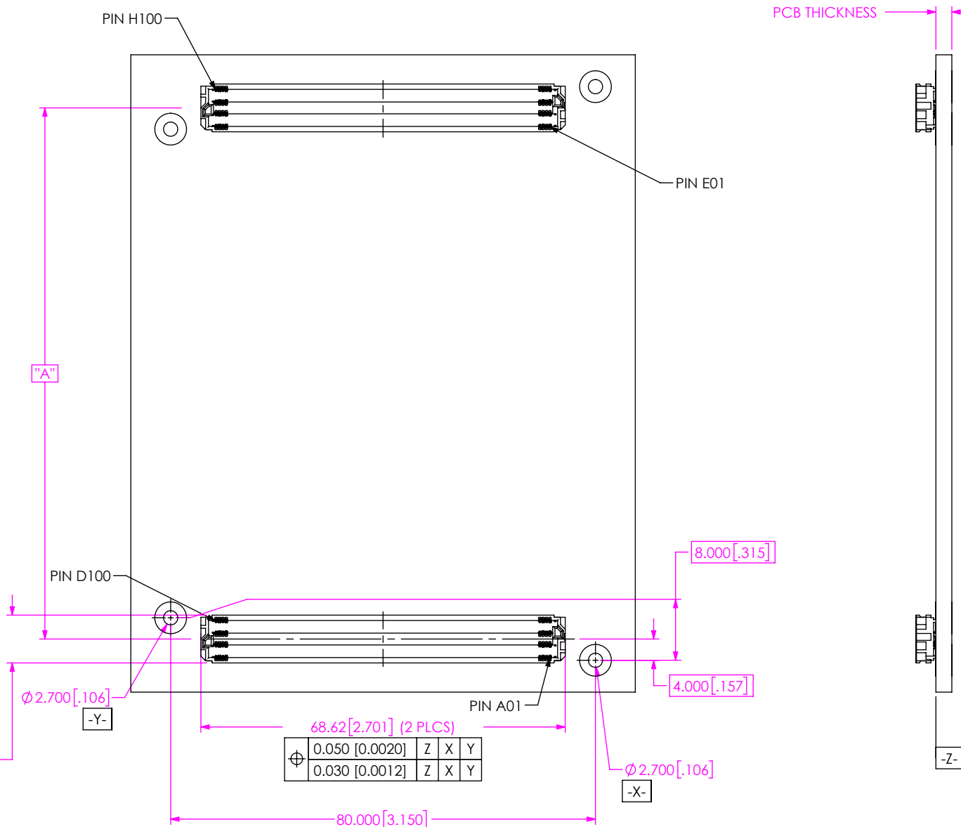
FIG 7 COM-HPC® ASSEMBLY APPLICATION (RECOMMENDED ASP-209946-02 LAYOUT FOR COM-HPC®)
