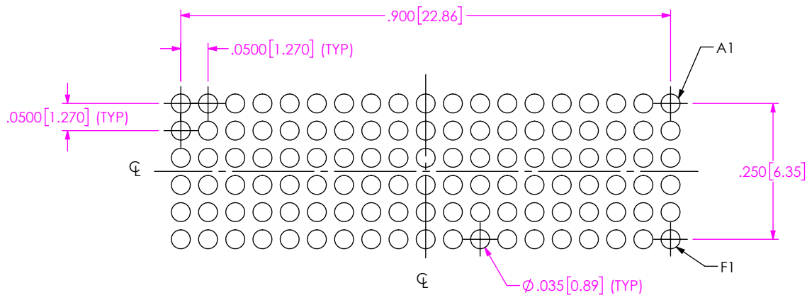
RECOMMENDED STENCIL LAYOUT (ALL DIMENSIONS ARE SYMMETRIC ABOUT THE CENTERLINE)
