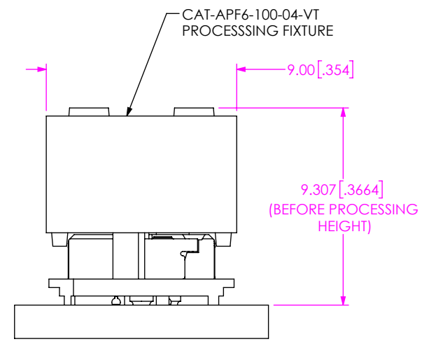
PROCESSING VIEW DIMENSION INDICATES CONNECTOR/FIXTURE HEIGHT ON PCB TO GUARANTEE ENOUGH REFLOW OVEN WORKING SPACE. DIMENSION, PCB THICKNESS, AND THE HEIGHT OF THE COMPONENTS ON THE OTHER SIDE OF THE BOARD NEED TO BE CONSIDERED.
