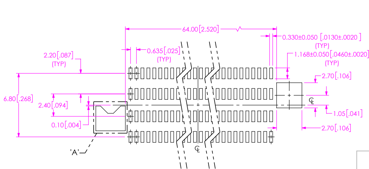
RECOMMENDED PCB LAYOUT ALL DIMENSIONS SYMMETRIC ABOUT CENTERLINE (ALL DIMENSIONS FOR REFERENCE ONLY)
