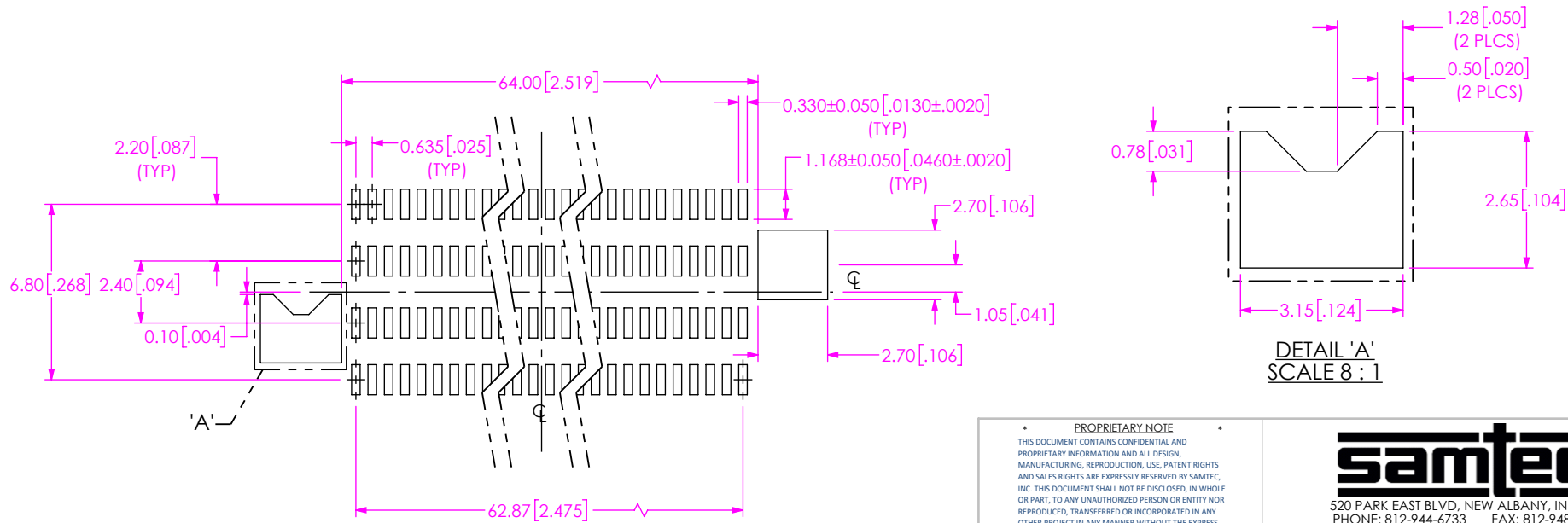
RECOMMENDED STENCIL LAYOUT ALL DIMENSIONS SYMMETRIC ABOUT CENTERLINE (STENCIL TO BE 0.125[.0050] THICK)
