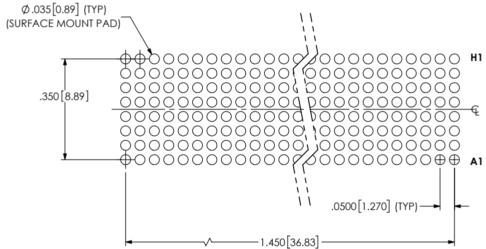
RECOMMENDED STENCIL LAYOUT ALL DIMENSIONS SYMMETRIC ABOUT CENTERLINE STENCIL TO BE .0060 THICK
