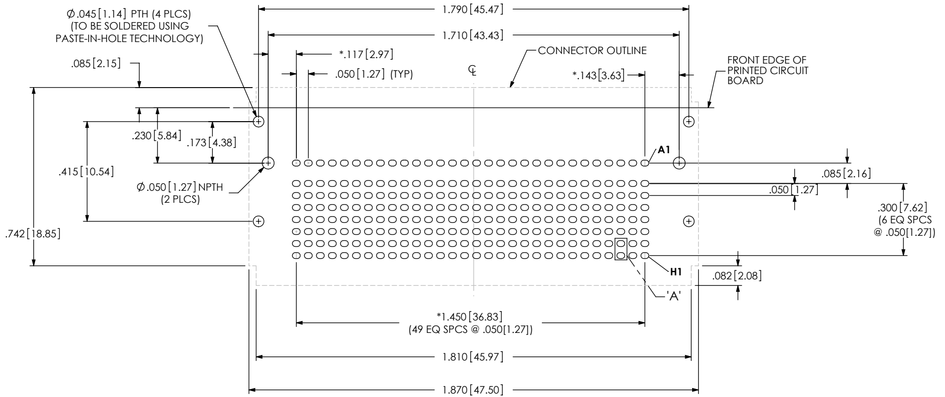
RECOMMENDED PCB LAYOUT ALL DIMENSIONS ARE SYMMETRIC ABOUT THE CENTERLINE EXCEPT "*" DIMENSIONS)
