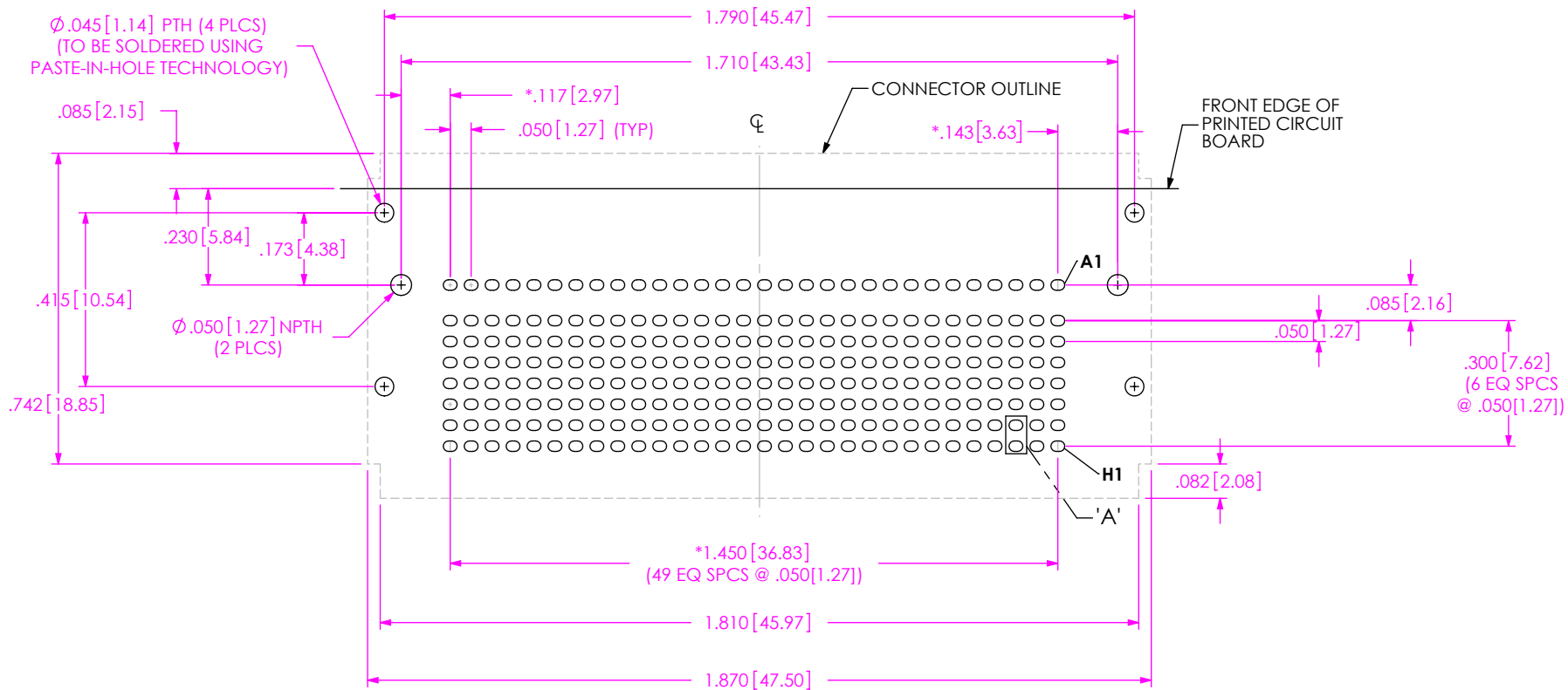
RECOMMENDED PCB LAYOUT ALL DIMENSIONS ARE SYMMETRIC ABOUT THE CENTERLINE EXCEPT "*" DIMENSIONS)
