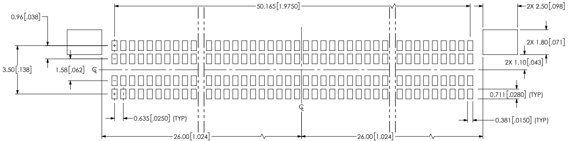
RECOMMENDED STENCIL LAYOUT ALL DIMENSIONS SYMMETRIC ABOUT CENTERLINE (STENCIL TO BE 0.127 [0.0050] THICK)
