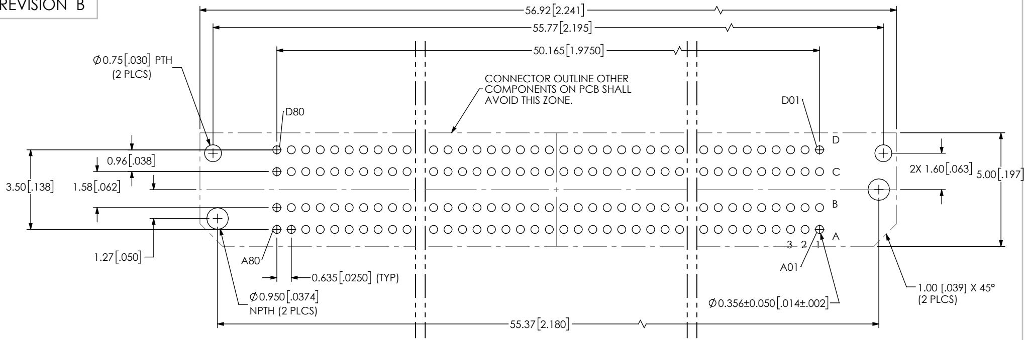
RECOMMENDED PCB LAYOUT ALL DIMENSIONS SYMMETRIC ABOUT CENTERLINE (ALL DIMENSIONS FOR REFERENCE ONLY)
