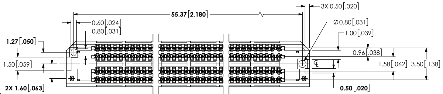
FIG 1 (ASP-240412-XX SHOWN)
