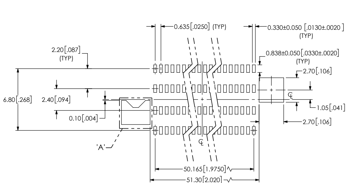
RECOMMENDED STENCIL LAYOUT ALL DIMENSIONS SYMMETRIC ABOUT CENTERLINE (STENCIL TO BE 0.125[.0050] THICK)
